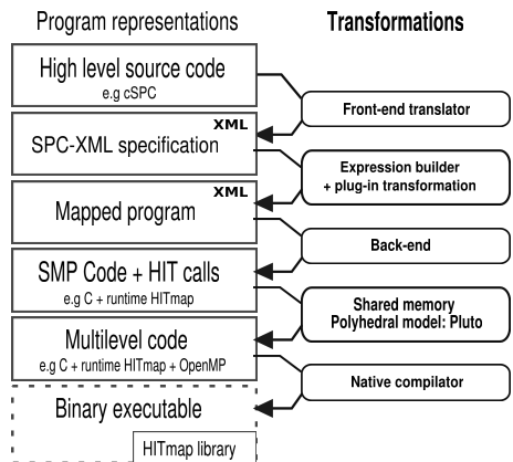
Figure 1: Structure of the Trasgo transformation framework.
