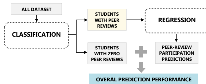
Fig. 2. The components of the ensemble method.
