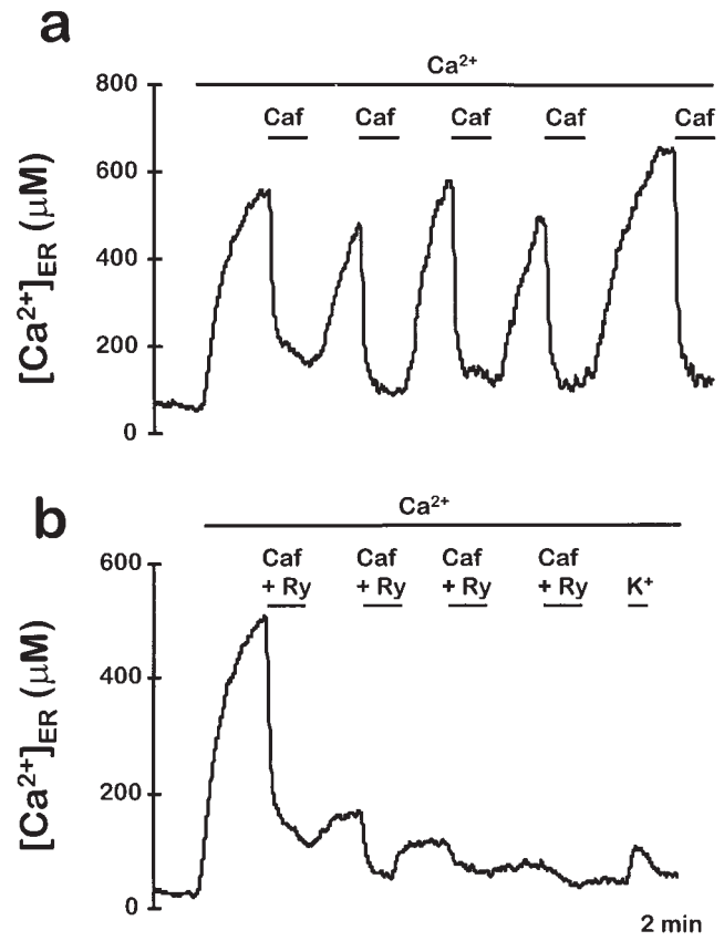
Figure 2. Use-dependent inhibition of ER refilling by ryanodine. The ER was refilled by perfusing with medium containing 1 mM \text{Ca}^{2+} . Then, several consecutive stimulations with 50 mM caffeine were performed as indicated, either in the absence (a) or in the presence (b) of 10 \mu\text{M} ryanodine. In b, standard medium containing 70 mM KCl (replacing an equimolar amount of NaCl) was perfused when indicated ( \text{K}^{+} ). Other details are as in Fig. 1.
