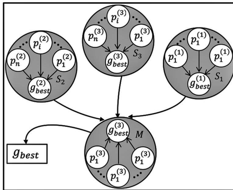
Figure 7. Flow chart of the cooperative PSO algorithm.
