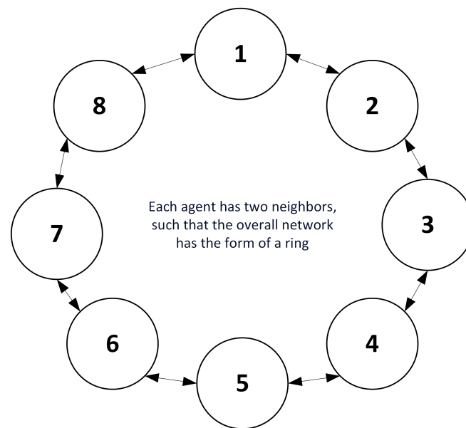
Figure 4. Ring topology PSO algorithm.
