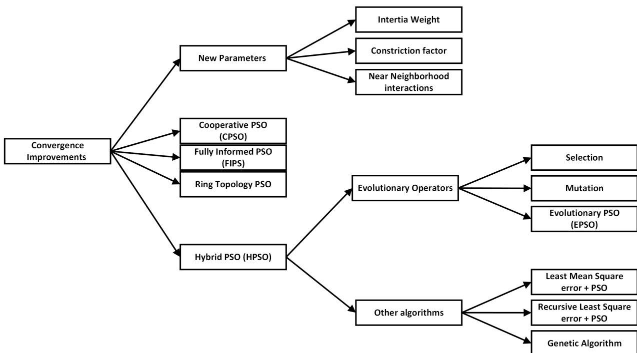
Figure 3. Convergence improvements of different variants of PSO.
