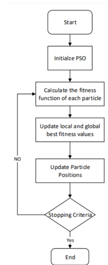
Figure 1. Flow chart of standard PSO algorithm.
