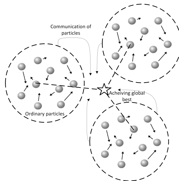
Figure 5. Dynamic multi-swarm PSO.
