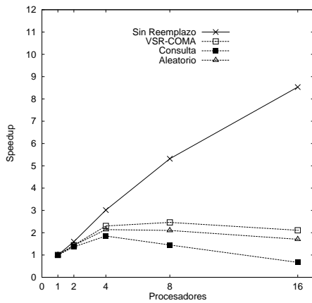
(c) Radix
