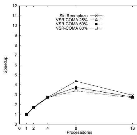
(f) Radiosity
