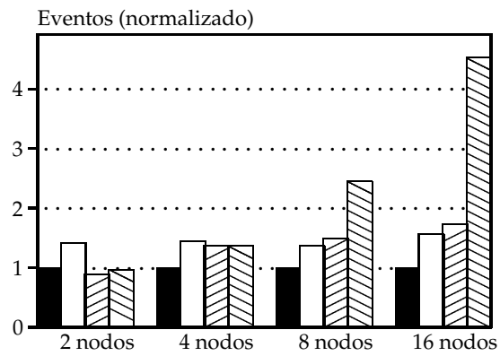
(a) FFT
