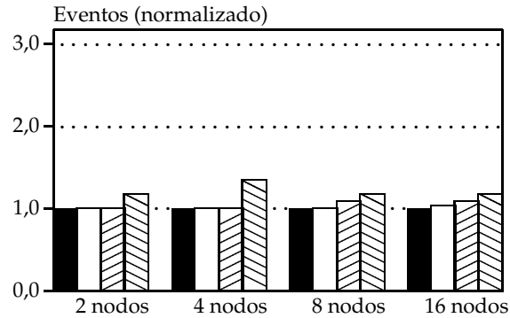
(a) FFT
