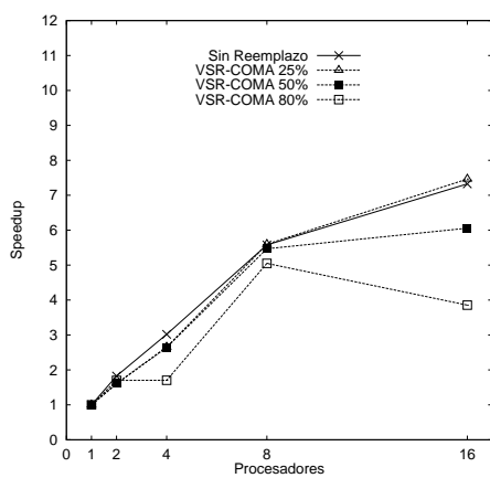
(e) Ocean
