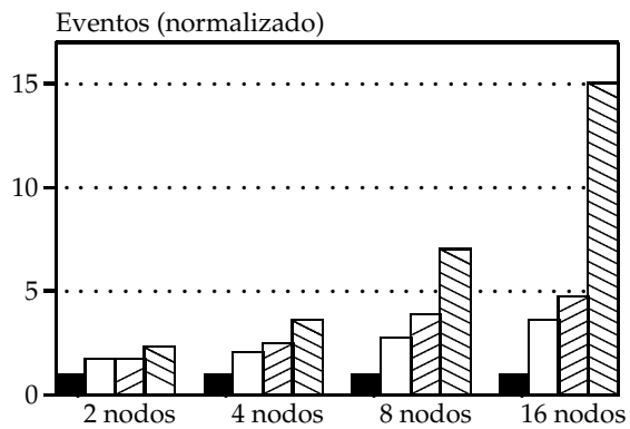
(c) Radix
