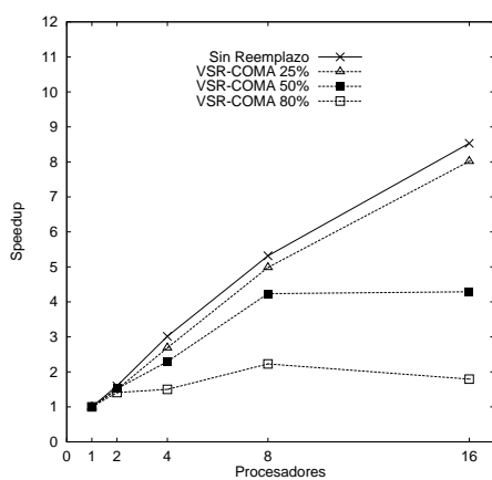
(c) Radix
