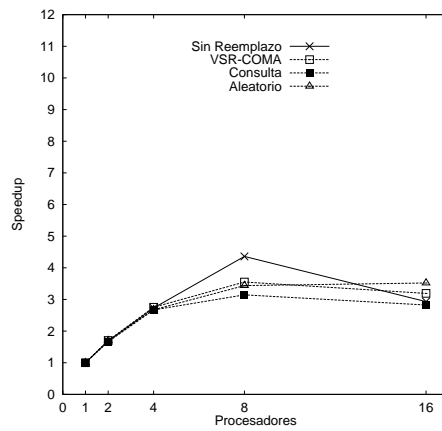
(f) Radiosity
