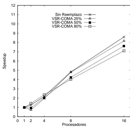
(a) FFT
