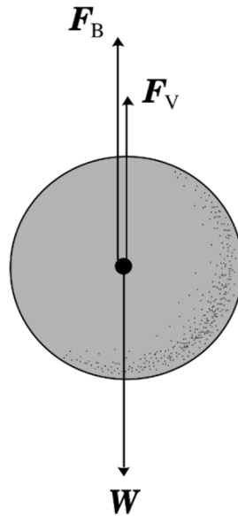
Figure 9. Schematic of the forces involved in the motion of a particle in a fluid, where F_B is the buoyant force, F_v is the viscous force (drag force) and W is the weight of the particle.
