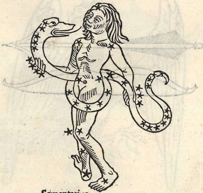
Serpentarius
