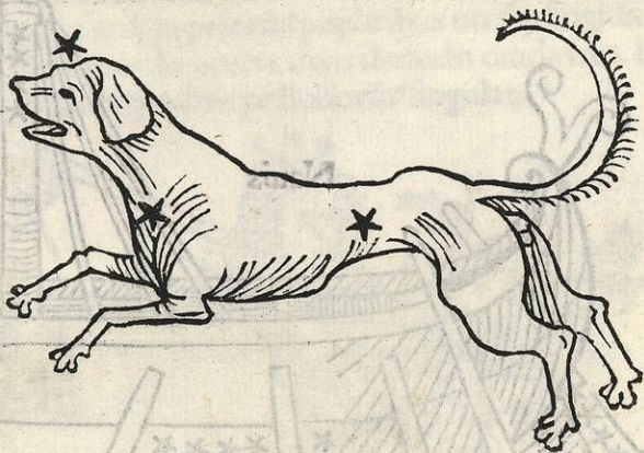
Canis minor
