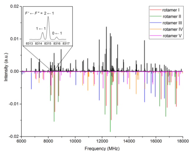
Figure 1. Broadband rotational spectrum of serinol in the 6-18 GHz frequency region. The upper trace shows the experimental spectrum, the lower trace is a simulation with the fitted rotational parameters and the experimental abundances. The inset shows the quadrupole coupling splitting of the 1_{1,0} \leftarrow 0_{0,0} transition of rotamer I .
