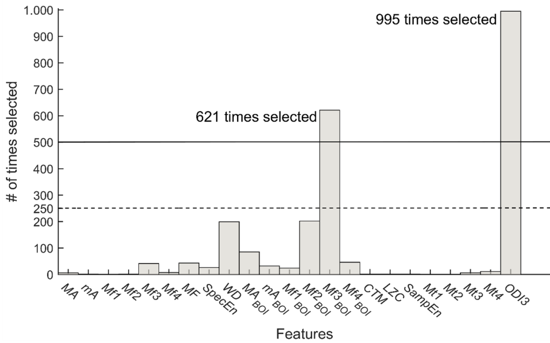
Supplemental Figure 2S. Histogram with the number of times each feature was selected after the bootstrap method.
