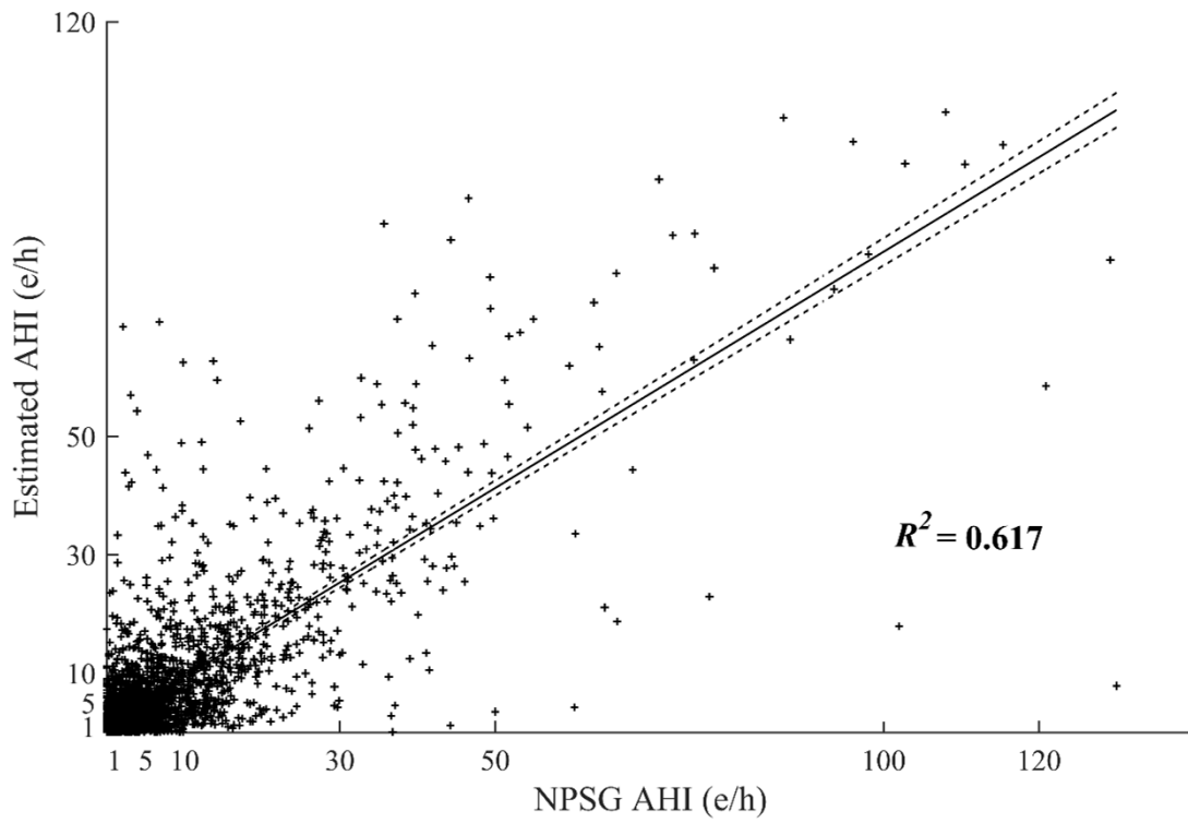
Supplemental Figure 4S. Scatter plot of the NPSG AHI and estimated AHI. The regression line and corresponding 95% confidence interval and R^2 statistic are also included.
