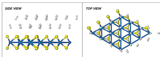
Figure 4. Top and side views of the optimized structure for two full layers of H 2 molecules adsorbed on top of a WS 2 layer. Blue, golden and white spheres represent W, S and H atoms, respectively.
