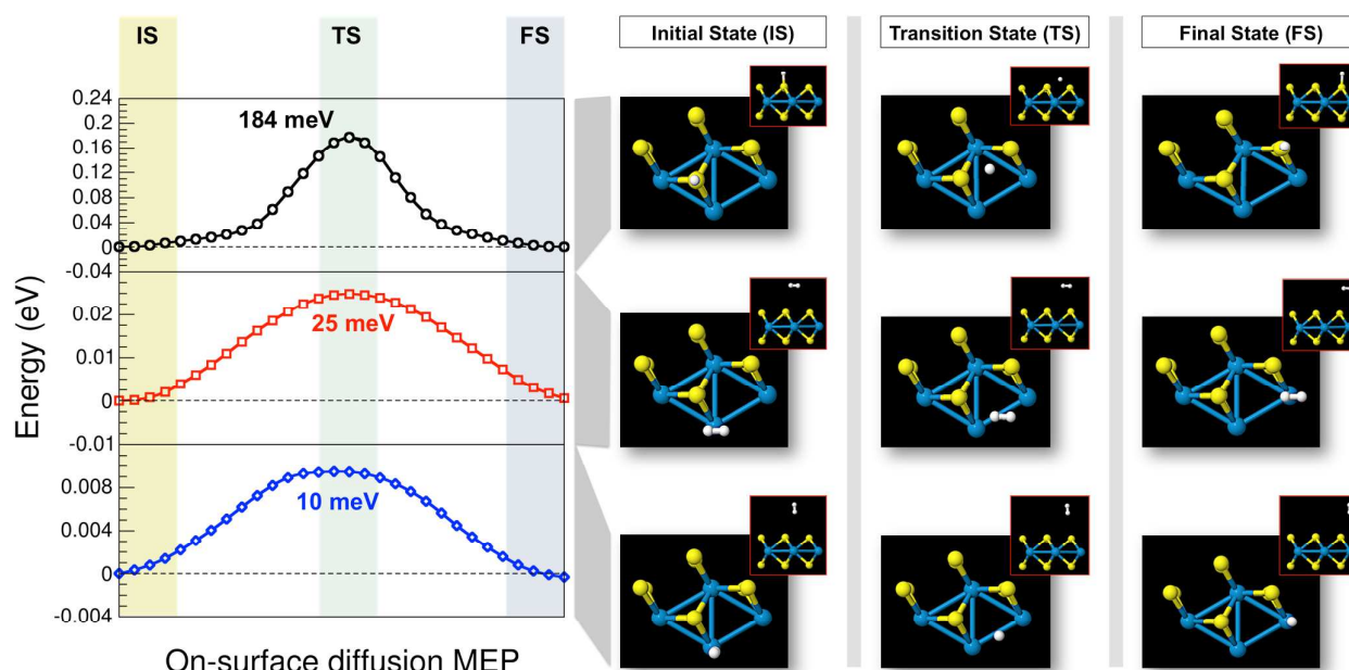
Figure 7. (Right panel) Top and side views of the initial state, IS, transition state, TS (corresponding to the maximum of the activation barrier), and final state, FS, for the diffusion of H (top panels) and H 2 (middle and bottom panels) on the WS 2 surface. (Left panel) Computed CI-NEB energy barriers along the diffusion minimum energy diffusion paths (MEPs). Blue, golden and white spheres represent W, S and H atoms, respectively.
