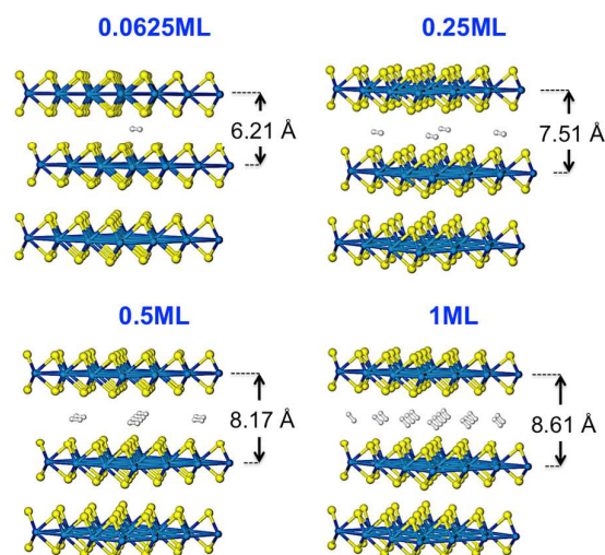
Figure 9. Optimal structures for intercalation of molecular hydrogen between the first and the second layers of the WS_2 trilayer for different H_2 content ( 0.0625 ML, 0.25 ML, 0.5 ML and 1 ML).
