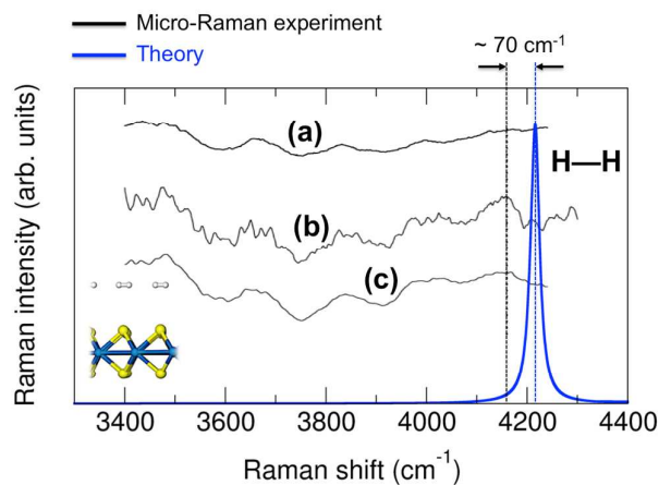
Figure 12. Black-solid lines are micro-Raman spectra of WS 2 nanoparticles: (a) non-hydrogenated, (b) plasma hydrogenated, (c) plasma hydrogenated and vacuum annealed up to 450 °C. A vertical line indicates the location of the H 2 peak at 4150 cm -1 . The Blue-solid line is the theoretical non-resonant Raman peak for 1 ML of H 2 molecules physisorbed on a planar WS 2 layer. A mismatch smaller than 70 cm -1 is found between experiment and theory.
