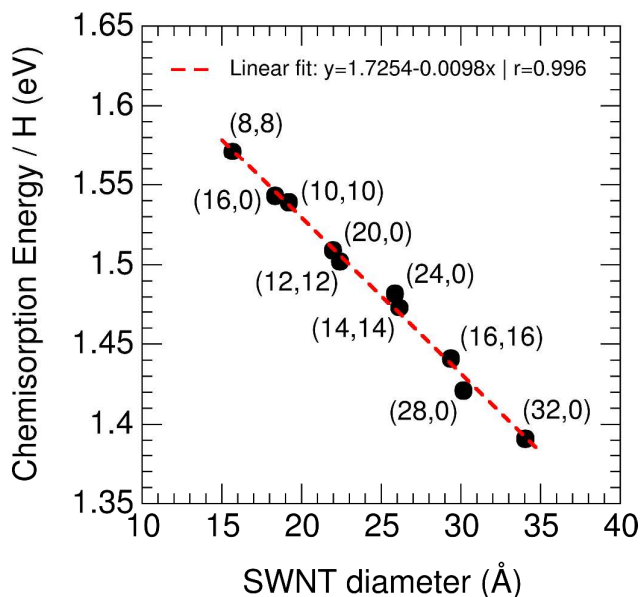
Figure 6. Chemisorption energy per H atom (in eV) as a function of the nanotube diameter (in Å), in the low coverage regime 0.0625 ML, for single-wall nanotubes: arm-chair (8,8), (10,10), (12,12), (14,14), (16,16), and zig-zag (16,0), (20,0), (24,0), (28,0), (32,0) nanotubes. The result of the linear regression is also shown in the figure.
