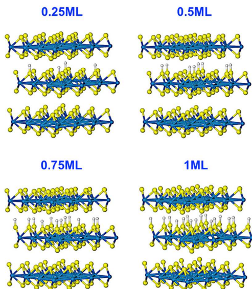
Figure 10. Optimal structures for the intercalation of atomic hydrogen between the first and the second layers of the WS 2 trilayer for different H content (0.25 ML, 0.5 ML, 0.75 ML and 1 ML). The H atoms are attached to S atoms belonging to the upper basal plane of the second WS 2 layer. Blue, golden and white spheres represent W, S and H atoms, respectively.
