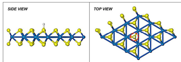
Figure 5. Top and side pictorial views of the optimized structure of an H atom chemisorbed on top of an S atom of a single WS 2 layer. Blue, golden and white spheres represent W, S and H atoms, respectively.
