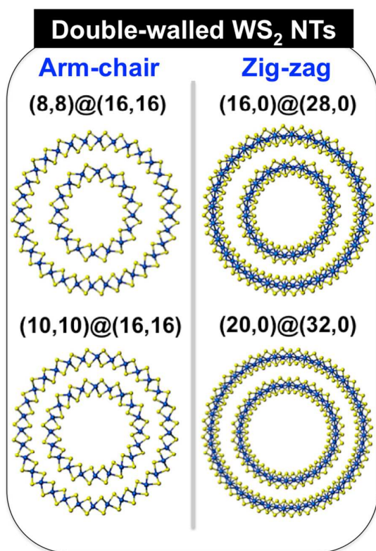
Figure 2. Optimized structures of the: (left) arm-chair (8,8)@(16,16) and (10,10)@(16,16), and (right) (16,0)@(28,0) and (20,0)@(32,0) double-walled WS 2 nanotubes. Blue and golden spheres represent W and S atoms, respectively.
