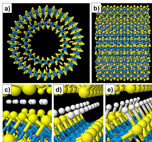
Figure 11. Initial state in three different views, panels (a), (b) and (c), and final state, panel (e), for H 2 molecules intercalated between the walls of a (10,10)@(16,16) nanotube. Eight rows of H 2 molecules have been intercalated, and for the nanotube fragment shown each row contains eight molecules. Panels (c), (d) and (e) show three representative steps along the spontaneous H 2 dissociation. In the (c), (d) and (e) panels, the upper and bottom WS 2 layers correspond to the outer and inner nanotubes, respectively.
