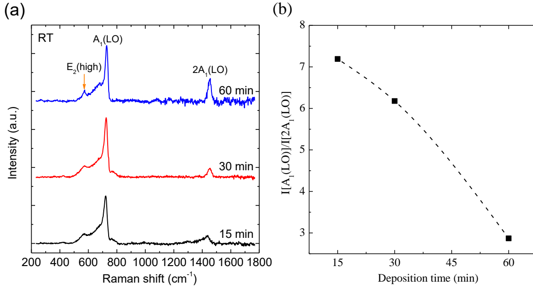
Figure 6. (a) Resonant Raman scattering spectra of nanoporous GaN samples grown at 15, 30 and 60 min excited with a 325 nm laser. (b) Intensity ratio of the A_1(\text{LO})/2A_1(\text{LO}) peaks vs deposition time for nanoporous GaN samples.
