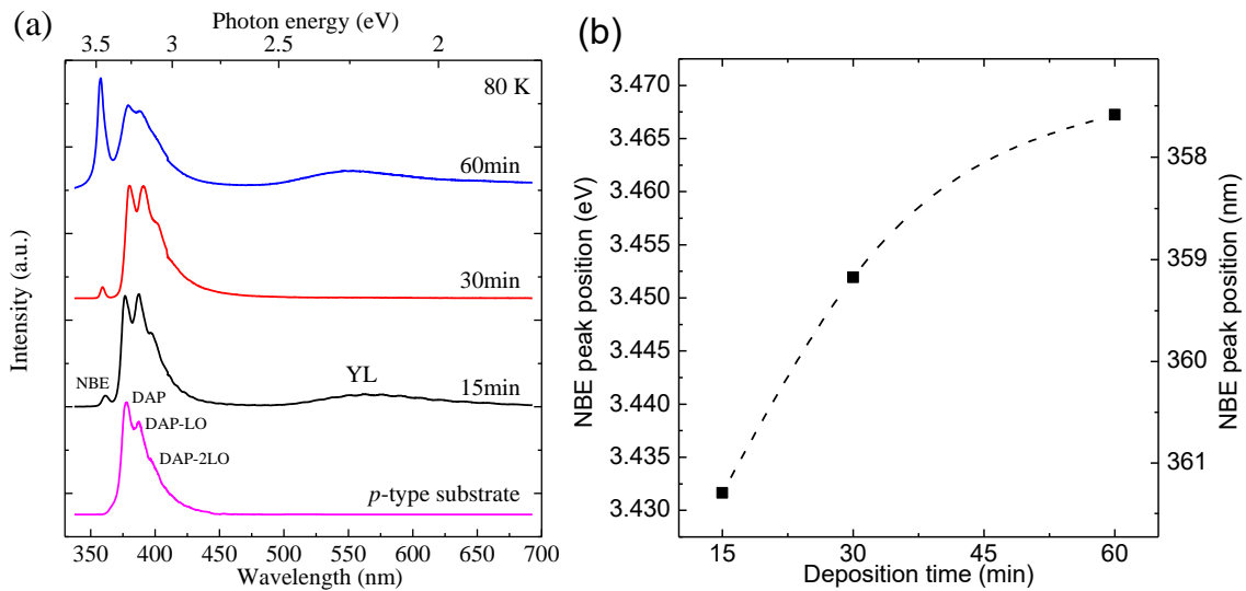
Figure 3. (a) PL spectra recorded at 80 K for nanoporous GaN samples grown at 15, 30 and 60 min. The spectrum of the non-porous p -type substrate on which the nanoporous layer are grown is also included. (b) Evolution of the position of the NBE band against the deposition time.
