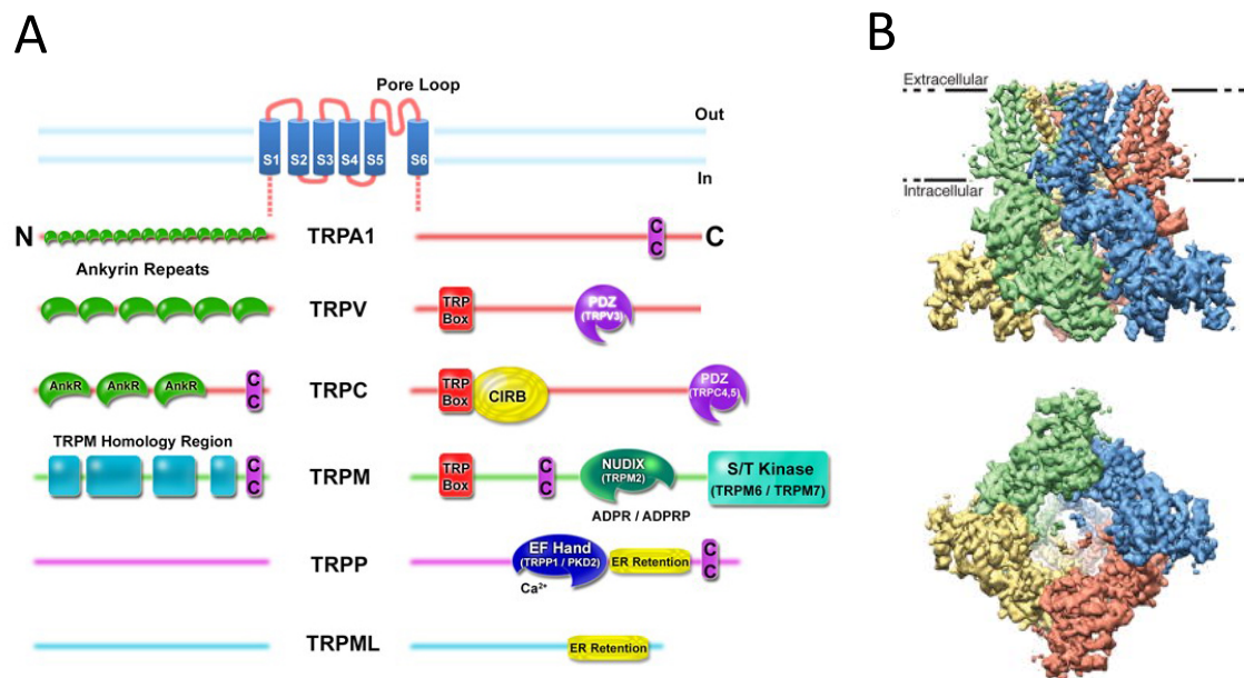
Figure 1.7. Topological structure of TRP channels and Cryo-EM reconstruction of TRPM8 channel. (A) TRP channel monomers have six transmembrane topology (S1-S6) with a pore loop between S5 and S6. The cytoplasmic N- and C-termini contain different structural and functional elements as indicated for each subfamily. Some of the sensory TRP channels such as TRPA1 and TRPV family contain multiple ankyrin repeats at their amino termini while TRPM family contain a homology region (modified from Clapham, D.E., 2003). (B) Cryo-EM reconstruction of the TRPM8 channel (Yin et al. , 2018).
