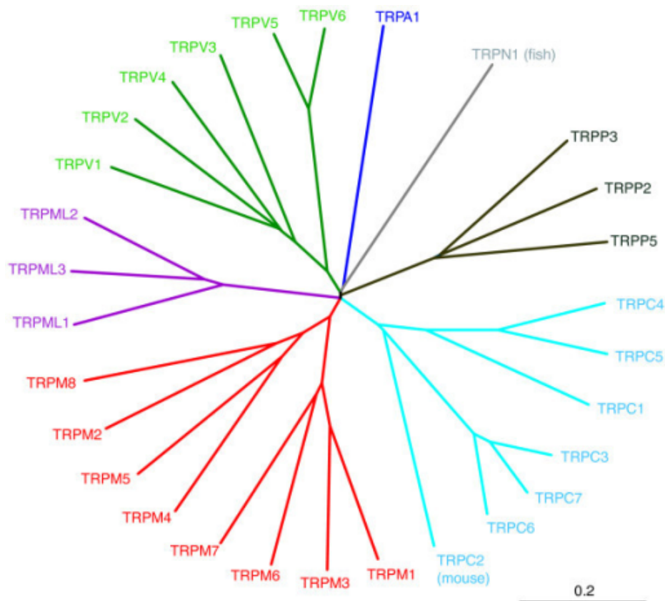
Figure 1.6. Phylogenetic tree of the TRP family of cation channels showing the classification into six subfamilies: TRPA (Ankyrin), TRPP (Polycystin), TRPM (Melastatin), TRPC (Canonical), TRPML (MucoLipin) and TRPV (Vanilloid) (Nillius, B. et al , 2011)
