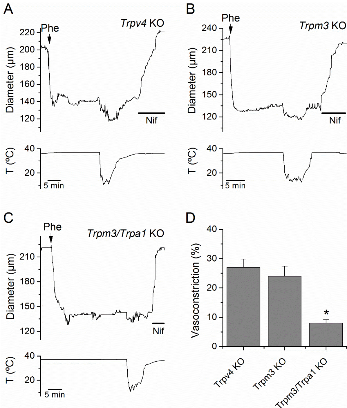
Figure 5.3. Cold-induced vascular responses are not dependent on TRPV4 or TRPM3. (A) Cold stimulation induces vasoconstriction in Trpv4 KO (A) and Trpm3 KO (B) plantar arteries. (C) Reduced effect of cold in Trpm3/Trpa1 KO plantar arteries. (D) Mean values of the effect in response to cold in plantar arteries from Trpv4 KO (n = 4), Trpm3 KO (n = 4) and Trpm3/Trpa1 KO (n = 7; * p < 0.005 ).
