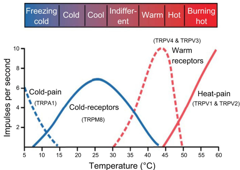
Figure 1.8. Frequencies at different skin temperatures of thermoreceptors, along with potential transient receptor potential (TRP) channels associated with receptor function (Tansey et al. , 2015).
