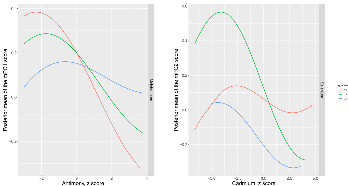
Fig. 1. Posterior mean of the difference in mPC1 and mPC2 scores by antimony and cadmium levels, when molybdenum and selenium, respectively, are fixed at its 10th, 50th and 90th percentiles.
