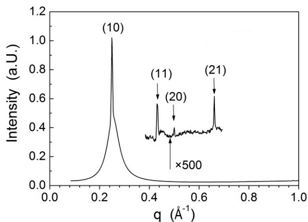
Figure 5. SAXS diffractogram (synchrotron) of adduct \mathbf{T}^2 at ca. 40 °C, after cooling from isotropic liquid.
