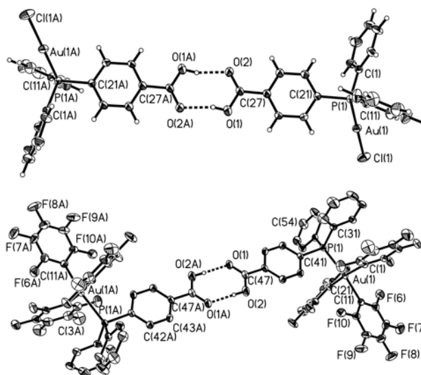
Figure 2. X-ray structures of dimers 4 (above) and 6 (below, H atoms omitted for clarity, except for the carboxylic group). Displacement ellipsoids are at 25% probability level.
