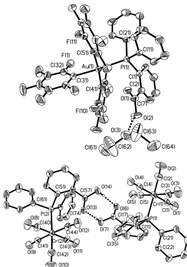
Figure 3. X-ray structure of compound 5 (above), and 9 (below). Displacement ellipsoids are at 30% probability level (H atoms omitted for clarity, except for the carboxylic group).
