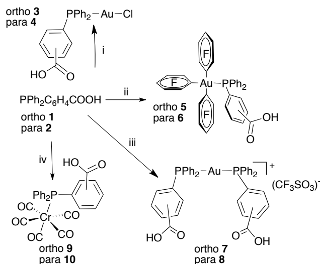
Scheme 1. Synthesis and molecular structures of the gold or chromium-organic acids 3–10 : i) [\text{AuCl}(\text{tht})] ; ii) [\text{Au}(\text{C}_6\text{F}_5)_3(\text{tht})] ; iii) \frac{1}{2} [\text{Au}(\text{tht})_2]\text{CF}_3\text{SO}_3 ; iv) [\text{Cr}(\text{CO})_6] + \text{Me}_3\text{NO} .
