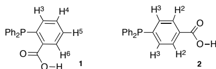
Figure 1. Structures of 2- and 4-diphenylphosphinobenzoic acids, and 1 H NMR labels.
