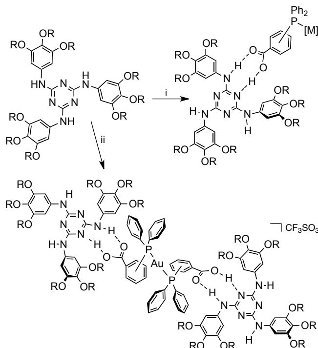
Scheme 2. Reactions for the synthesis of supramolecular triazine–metalloacid adducts, T^n . The H-bonding system is indicated by dashed lines. R = C_{10}H_{21} . The attempted syntheses are: i) reactions with compounds 1–6 , 9 and 10 ; ii) the same, with compounds 7 and 8 ).
