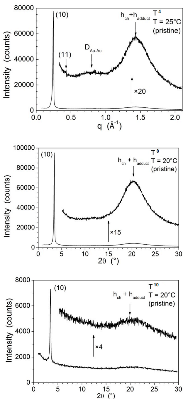
Figure 6. X-ray diffraction patterns for a) T^4 at 25^\circ\text{C} , b) T^8 at 20^\circ\text{C} and c) T^{10} at 20^\circ\text{C} .
