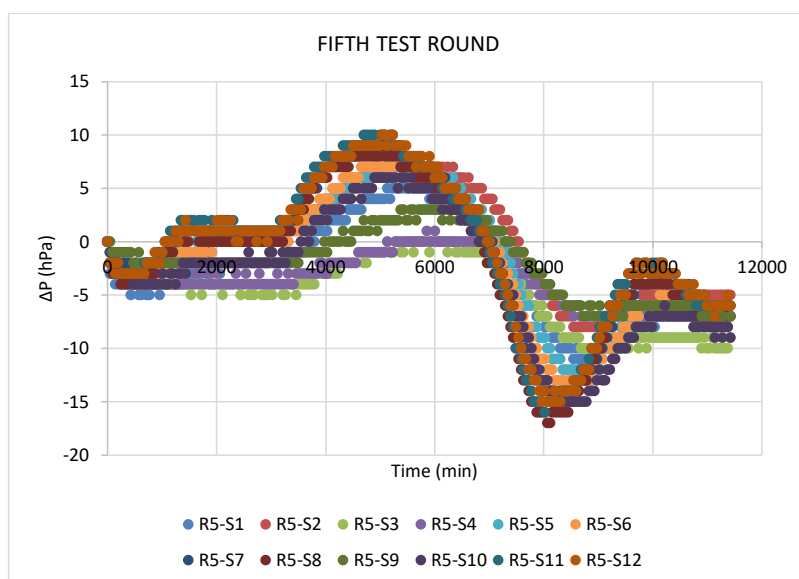
FIGURE 4.4.5 Graphical presentation of pressure change in the fifth test round
