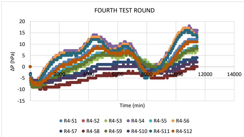
FIGURE 4.4.4 Graphical presentation of pressure change in the fourth test round
