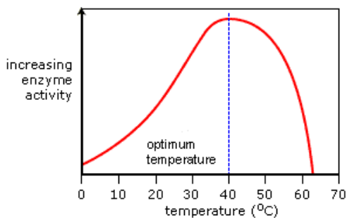
FIGURE 2.4.1. Relationship between enzyme activity and temperature ( http://www.bbc.co.uk/schools/gcsebitesize/science/add_aqa/proteins/proteinsrev3.shtml )
