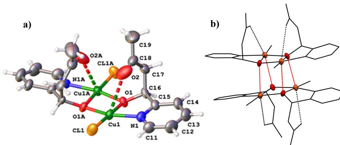
Figure 6. a) Structure of 3a , showing the atom numbering. Selected bond lengths (Å) and angles (°): Cu(1)-N(1) 1.988(2), Cu(1)-O(1) 1.929(2), Cu(1)-O(2) 1.954(2), O(1)-Cu(1)-N(1) 81.46(9), O(1)-Cu(1)-O(1A) 78.32(8), Cl(1)-Cu(1)-N(1) 99.47(7). b) Interaction of the two Cu_2O_2 rings through the alkoxide (highlighted in red) to give an overall octahedral geometry around each Cu center and the formation of a Cu_4O_4 central cage.
