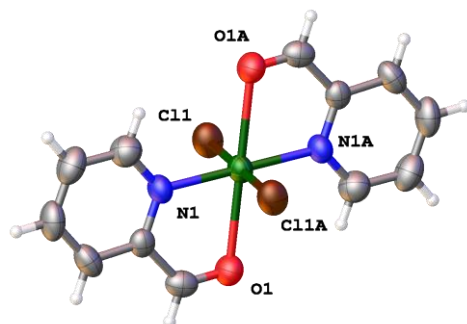
Figure 3. Perspective view of compound 2 showing the atom numbering. Selected bond lengths (Å) and angles (°): Cu(1)-Cl(1) 2.299(1), Cu(1)-N(1) 1.989(4), Cu(1)-O(1) 2.443(4), Cl(1)-Cu(1)-Cl(1A), Cl(1)-Cu(1)-Cl(1A) 180.00(1), N(1)-Cu(1)-N(1A) 180.00(1), Cl(1)-Cu(1)-N(1) 90.80(15), Cl(1)-Cu(1)-O(1) 90.80(15).
