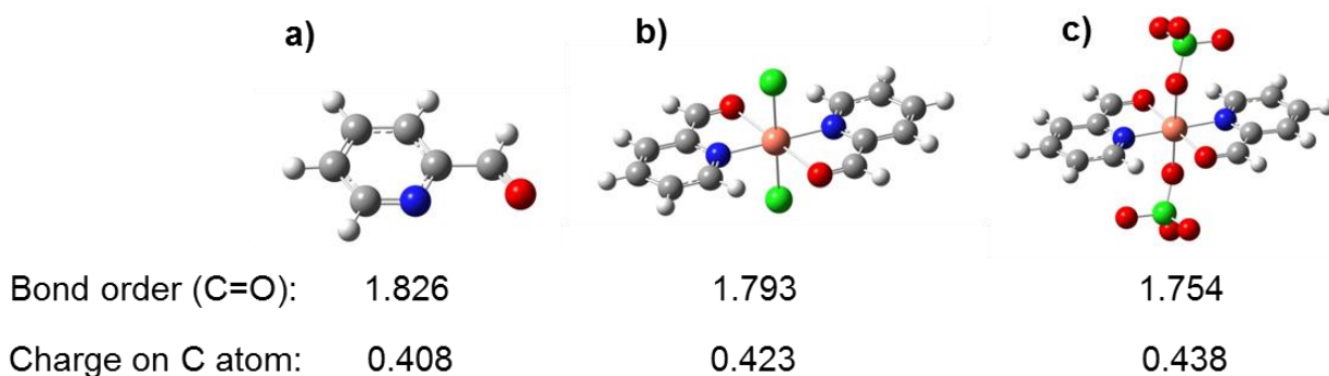
Figure 4: Optimized geometries, bond orders, and charge on the aldehyde carbon atom obtained from DFT calculations for (a) free pyca; (b) \text{CuCl}_2(\text{pyca})_2 , complex 2 ; and (c) \text{Cu}(\text{ClO}_4)_2(\text{pyca})_2 .
