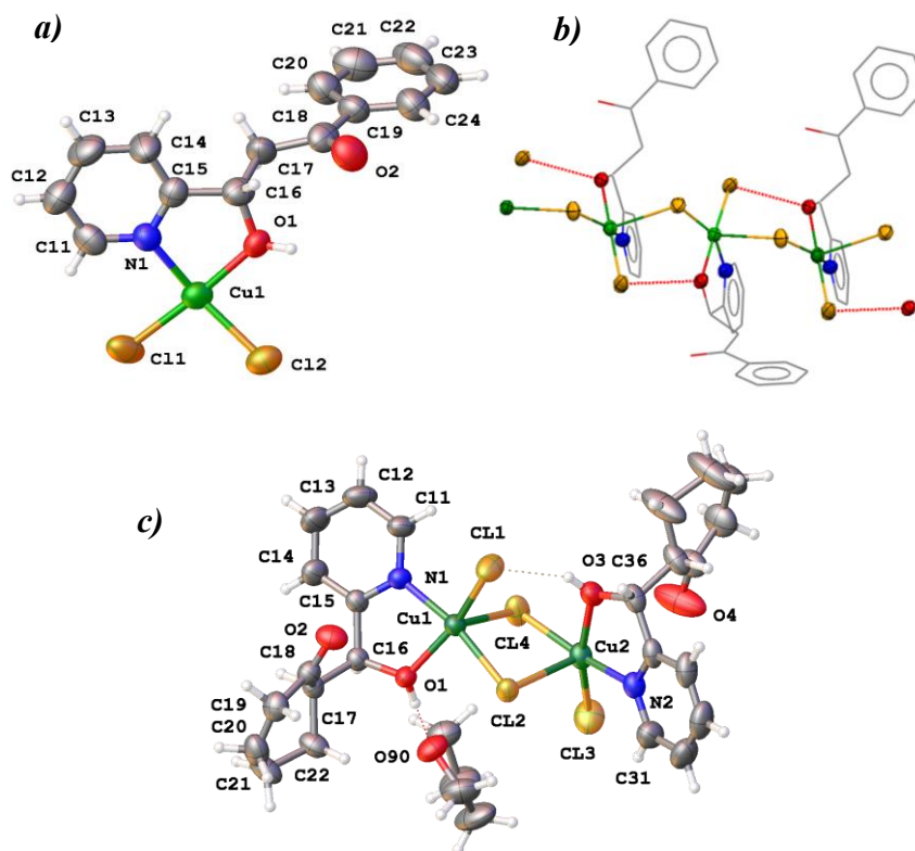
Figure 5. a) Structure of 1b showing the atom numbering. Selected bond lengths (Å) and angles (°): Cu(1)-Cl(2) 2.260(2), Cu(1)-Cl(1) 2.255(2), Cu(1)-Cl(1A) 2.741(2), Cu(1)-N(1) 2.016 (6), Cu(1)-O(1) 2.009(5), N(1)-Cu(1)-O(1) 80.0(2) Cl(1)-Cu(1)-Cl(2) 95.75(8), Cl(1)-Cu(1)-Cl(1A) 91.71 (7). H-Bonding: O(1)-H(1) 0.938(0), O(1)...O(2) 3.205(8), H(1)...O(2) 2.696(6), O(1)-H(1)...O(2) 114.9(4). b) Polymeric structure of 1b through Cl(2)...Cu(1) interactions between adjacent complexes, so that the geometry around Cu can be considered square pyramidal. c) Structure of 1c showing the atom numbering. Selected bond lengths (Å) and angles (°): Cu(1)-Cl(1) 2.225(2), Cu(1)-Cl(2) 2.259(1), Cu(1)-Cl(4) 2.756(1), Cu(1)-N(1) 1.996 (3), Cu(1)-O(1) 2.036(3), Cu(1)-Cu(2) 3.5597(7), N(1)-Cu(1)-O(1) 80.42(13) Cl(1)-Cu(1)-Cl(2) 97.33(5), Cl(2)-Cu(1)-Cl(4) 87.06 (4). H-Bonding: O(1)-H(1) 0.938(0), O(1)...Cl(3) 3.092(3), H(1)-Cl(3) 2.205(1), O(1)-H(1)...Cl(3) 157.3(2), O(3)-H(3) 0.938(0), O(3)...O(90) 2.565(4), H(3)...O(90) 1.640(3), O(3)-H(3)...O(90) 168.1(2).
