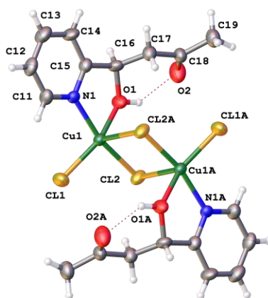
Figure 2. Structure of 1a showing the association into dimers in solid state through Cu-Cl interactions. Selected bond lengths (Å) and angles (°): Cu(1)-Cl(1) 2.216(2), Cu(1)-Cl(2) 2.254(1), Cu(1)-Cl(2A) 2.757(2), Cu(1)-N(1) 2.008(4), Cu(1)-O(1) 1.996(3), N(1)-Cu(1)-O(1)
