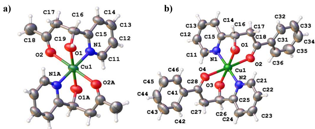
Figure 7. a) Structure of the dication in 4a , showing the atom numbering. The two ClO 4 anions have been omitted for clarity. Selected bond lengths (Å) and angles (°): Cu(1)-N(1) 1.945(4), Cu(1)-O(1) 2.038(3), Cu(1)-O(2) 2.283(4), O(1)-Cu(1)-N(1) 82.18(2), O(2)-Cu(1)-N(1) 86.47(2), O(1)-Cu(1)-O(2) 79.54(2). b) Structure of the dication in 4b , showing the atom numbering. The two ClO 4 anions have been omitted for clarity. Selected bond lengths (Å) and angles (°): Cu(1)-N(1) 1.966(5), Cu(1)-O(1) 1.904(4), Cu(1)-N(2A) 1.978(5), Cu(1)-O(1A) 1.948(4), Cu(1)-O(2A) 2.336(4), Cu(1)-Cu(1A) 2.948(2), N(1)-Cu(1)-N(2A) 106.4(2), N(1)-Cu(1)-O(1) 82.21(2), O(1)-Cu(1)-O(1A) 80.14(2).
