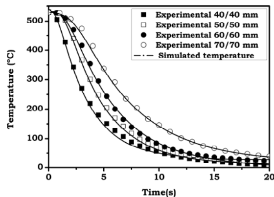
Figure 9. Predicted cooling curves and experimental ones obtained for solid cylinders of different dimensions.
