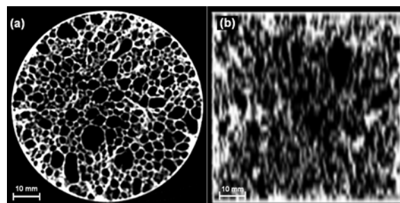
Figure 4. Tomographic slices of the 70/70 ( 690 \text{ kg/m}^3 ) foam: (a) XY-plane and (b) ZX-plane.
