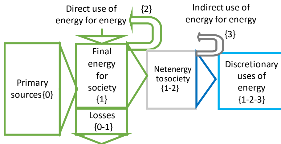
Figure 1. Energy flux from primary material sources of energy {0} to discretionary uses of energy. EROI_{st} = \{0\}/g\{2\} (EROI standard, being “g” a correction factor to convert “primary” to final). EROI_{final} = \{1\}/\{2'\} (EROI final, where {2'} includes the direct use of energy to bring it to the user) and EROI_{ext} = \{1\}/(\{2'+3\}) (EROI extended, all the terms at final and user phase). Note that the relevant energy for a society is the blue box (discretionary uses of energy), but primary sources of energy, and the other boxes, are relevant for environment issues because they are always taken/used in the biosphere (see reference [3] for more details).
