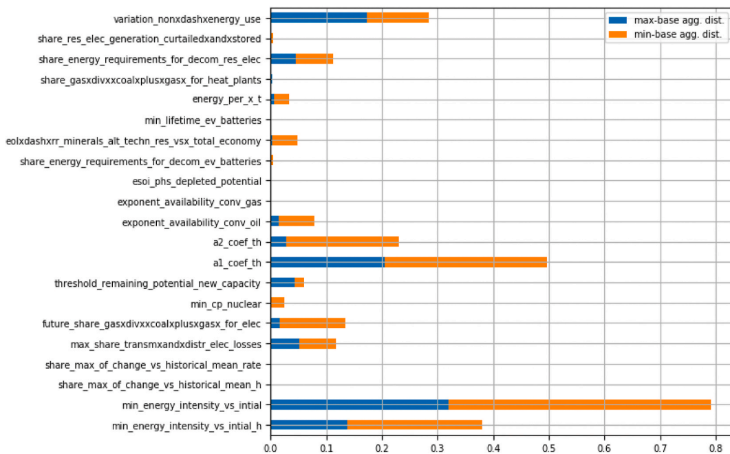
Fig. 7. Distances between the simulation results obtained with the minimum and nominal (base in the legend) values and the maximum and nominal (base in the legend) values aggregated for all output parameters, and normalised by the percentage change of the perturbed parameter with respect to the base value. Larger values correspond to greater distances between the compared simulation results.
