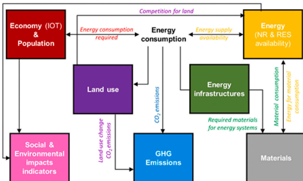
Fig. 1. Graphical representation of the modules of the MEDEAS models [35].
