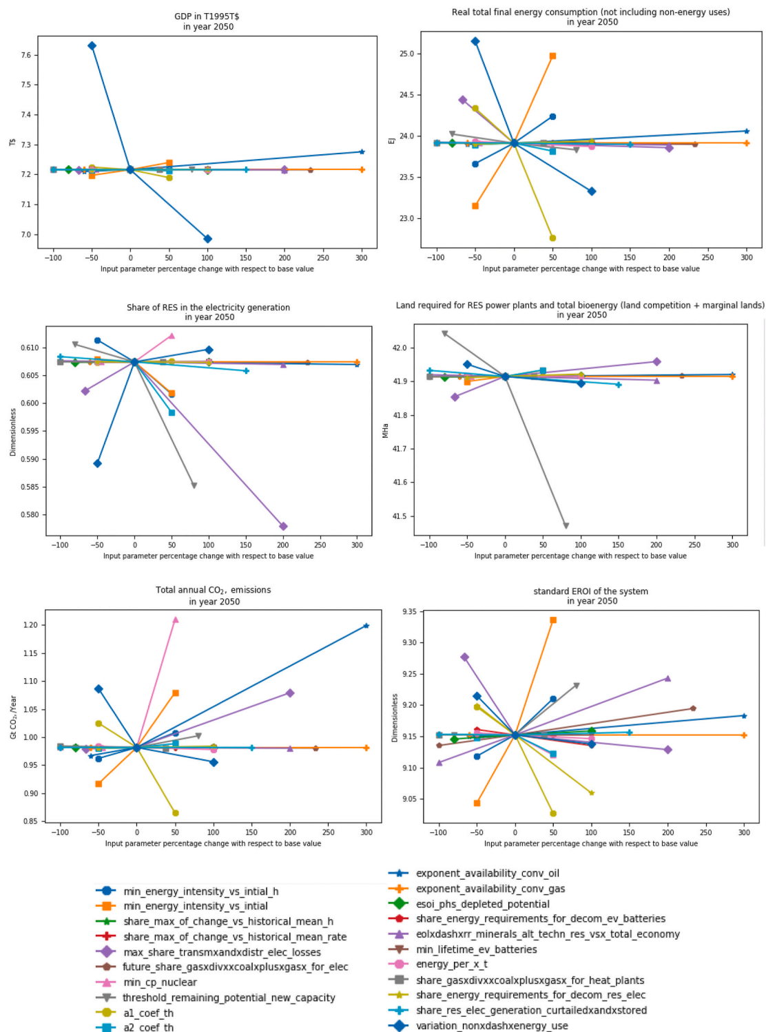
Fig. 6. From top-left to bottom-right, values of the GDP, final energy consumption, share of RE in electricity generation, land requirements for RE power plants, annual CO 2 emissions and standard EROI of the system in 2050, obtained by changing the model parameter values by a specified percentage with respect to the base value (x axis).
