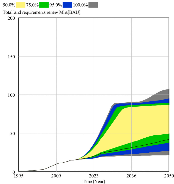
Fig. 5. Confidence bounds for the total land required by renewable power plants (in Mha) for the 1000 Monte Carlo simulations.
