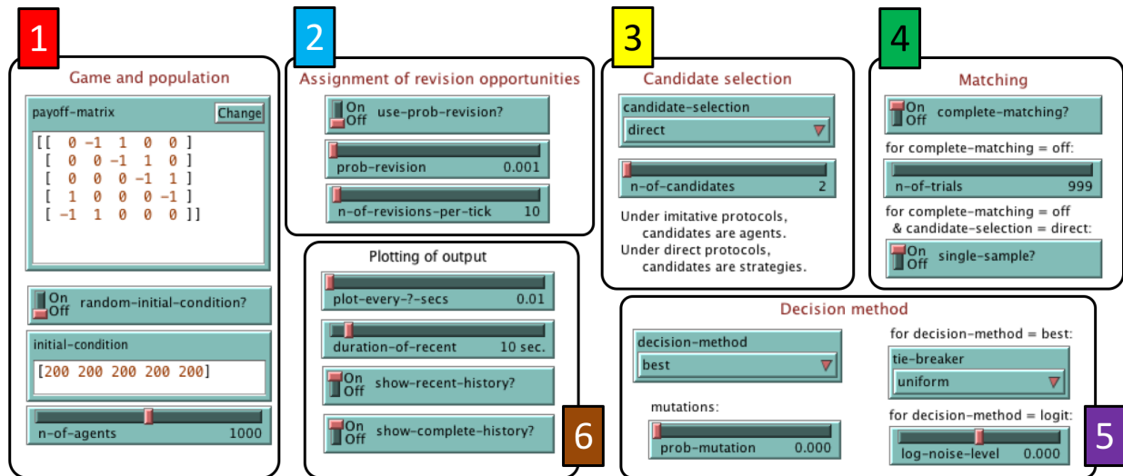
Figure 3: Main parameters in ABED-1pop.
