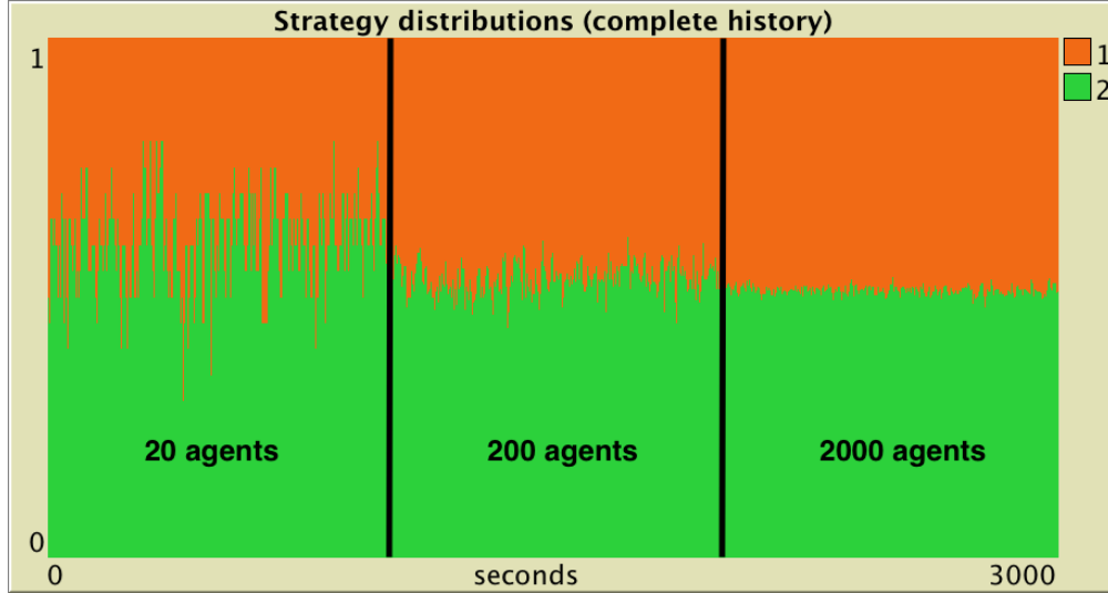
Figure 5: Time series of the population state in Hawk-Dove game under “imitate the best realization”. (Simulation parameters: Table 1 in the online appendix; hawk-dove.csv.)
