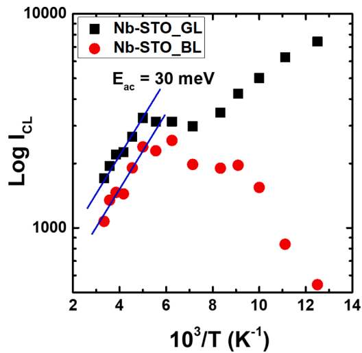
Fig. 10. BL and GL PL intensities as a function of temperature (Nb-doped sample).
