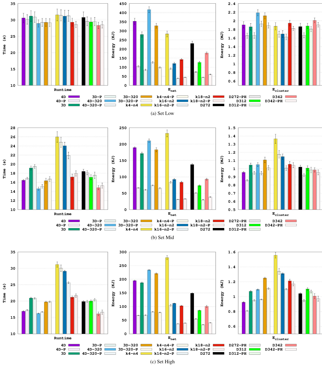
Fig. 5. Performance and energy evaluation for 256-node tori, fat-trees, and near-sized tori, fat-trees and dragonflies.
