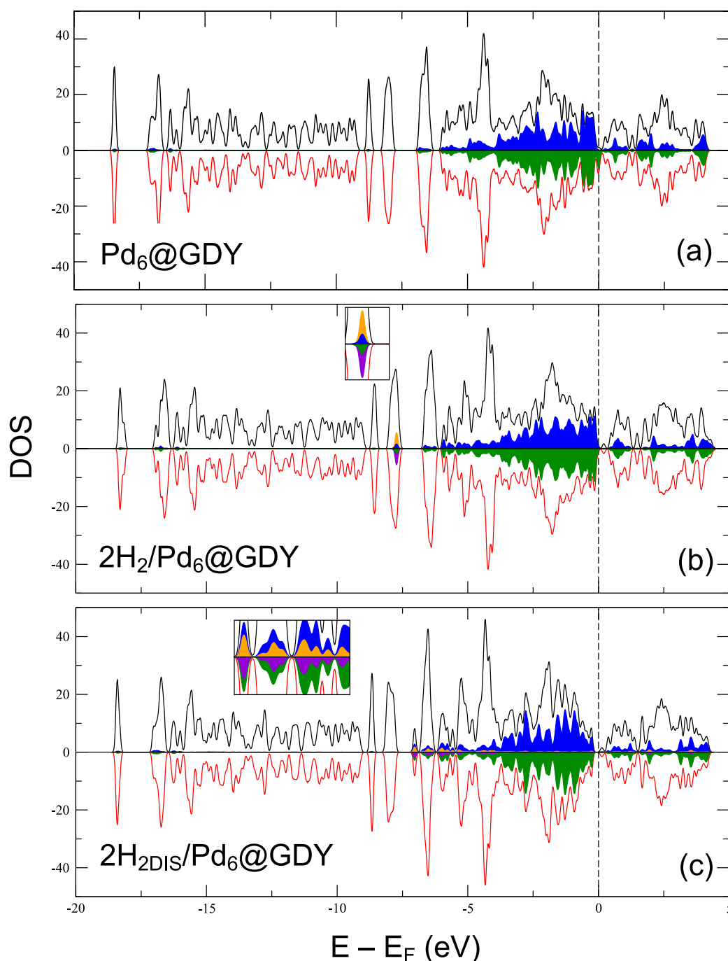
Figure 9. DOS of \text{Pd}_6\text{@GDY} , 2(\text{H}_2)/\text{Pd}_6\text{@GDY} , and 2(2\text{H})/\text{Pd}_6\text{@GDY} , separated in spin-up (black color) and spin-down (red color) components. Blue and green regions correspond to the DOS projected on the Pd atoms. Projections on H atoms are indicated in orange and purple.
