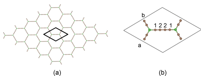
Figure 2. Left panel: honeycomb structure of BGDY. Right panel: unit cell and labeling of carbon atoms. Boron and carbon atoms are represented by green and brown spheres, respectively.
