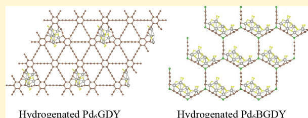
Hydrogenated Pd 6 GDY
