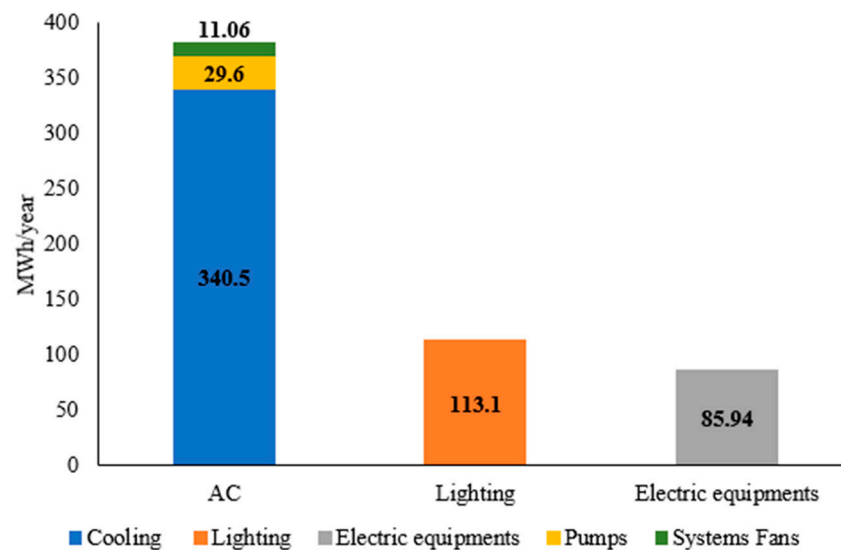
Figure 4. Distribution of the electrical energy consumption of the building Chiller technology.
