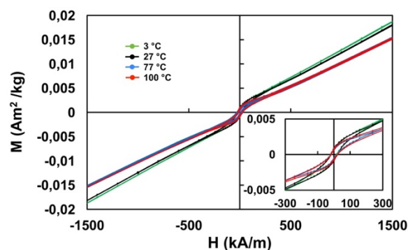
Figure 9. Field dependent magnetization curve of the nickel compound ( 5 ) at different temperatures.
