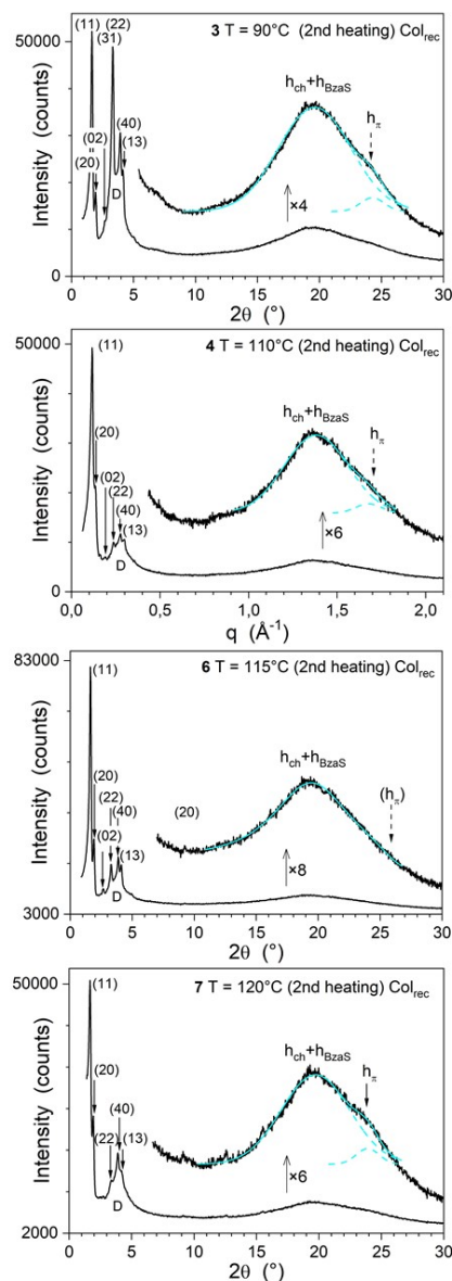
Figure 4. Representative S/WAXS patterns of the compounds in the mesophase. hk indexation of the small-angle peaks; h_{\text{ch}}+h_{\text{BzaS}} , undifferentiated liquid-like lateral distances between aliphatic chains and spacers, and benzylammonium-salt moieties, respectively; h_{\pi} , triphenylene stacking over short distances; D , short-range correlated periodicity from the supramolecular assembly. For 6 , the signal cannot be deconvoluted since the stacking signal ( h_{\pi} ) is too weak, if not nonexistent; its theoretical position (shown in brackets) is indicated by the dashed arrow.
