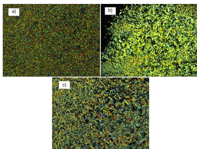
Figure 3. Optical polarizing microscopy photographs (x100, crossed polarizers) on cooling from the isotropic phase of: a) [TPh-NH 2 Et]Cl ( 3 ) at 87 °C; b) [TPh-NH 2 Et] 2 [CuCl 4 ] ( 4 ) at 109 °C; c) [TPh-NH 2 Et] 2 [NiCl 4 ] ( 5 ) at 112 °C.
