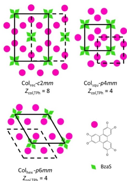
Figure 5. Illustration of the proposed 2D packing for the Col rec mesophase ( c2mm symmetry), and for the Col squ mesophase ( p4mm symmetry), and for the Col hex mesophase ( p6mm symmetry). The pink disks correspond to TP-based columns, and the green petals to BzaS-based aggregates; the aliphatic chains, occupying the white areas, are not shown for clarity.
