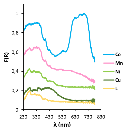
Figure 2. UV-Vis diffuse reflectance spectra of the TPh-NH 2 Et + salts in the solid state (diffuse reflectance) at 298 K (L = Cl - salt; M = [MCl 4 ] 2- salt).
