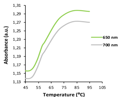
Figure 8. Absorbance change at \lambda = 650 nm and \lambda = 700 nm as a function of temperature.
