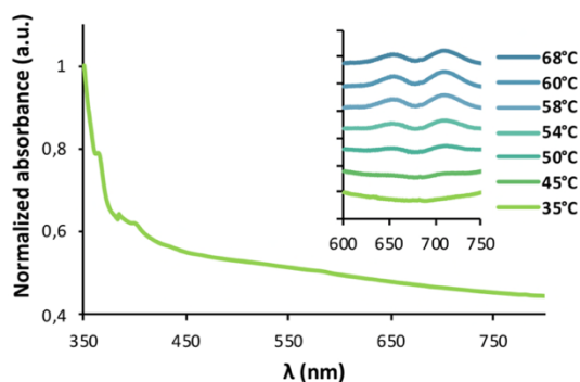
Figure 7. Electronic spectrum of [TPh-NH 2 Et] 2 [NiCl 4 ] ( 5 ) at 35 °C. Inset: spectral changes produced upon varying the temperature.
