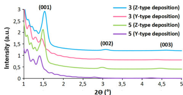
Figure 11. Low-angle X-ray diffractograms for the LB films of 3 and 5 .
