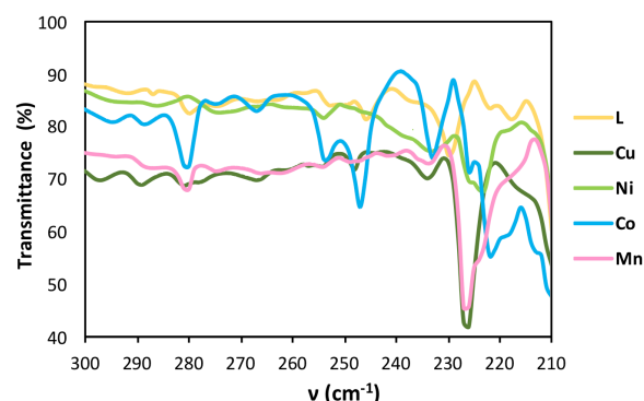
Figure 1. Far-infrared spectra of TPh-NH 2 Et + salts at 298 K (L = Cl - salt; M = [MCl 4 ] 2- salt).
