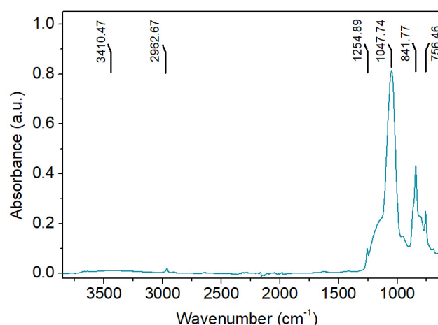
Figure 7-1-3: FTIR spectra of the Enova® Aerogel powder.
