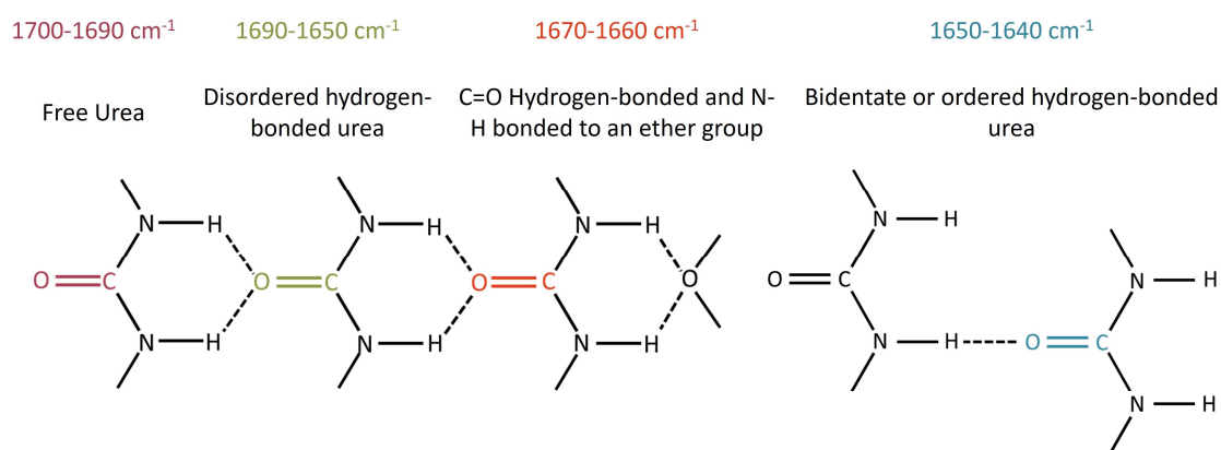
Figure 2-14: Characteristic frequencies of the urea groups generated during the blowing reaction including free urea and hydrogen-bonded urea [49,50,56-60].
