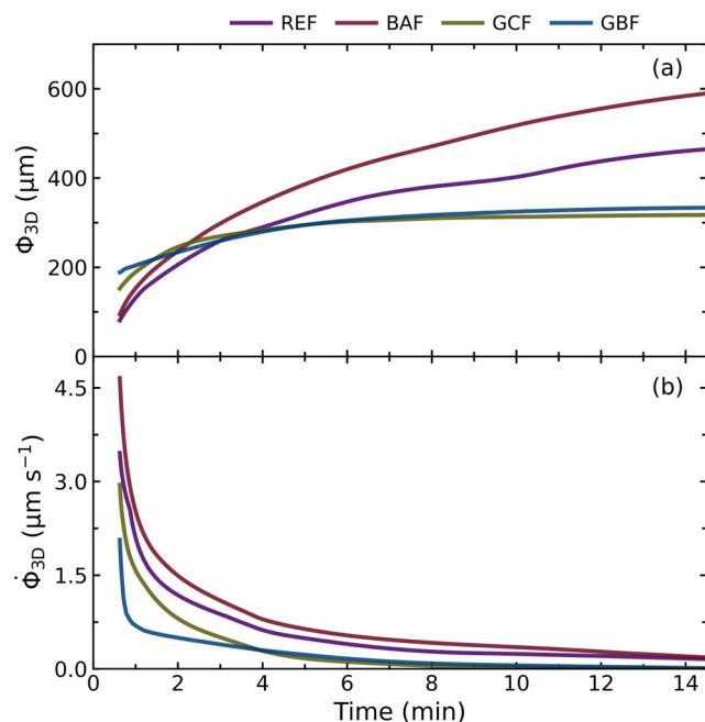
Figure 4-2-6: (a) Mean cell diameter and (b) rate of cell growth evolution with time calculated as the first derivate of the curves in (a)
