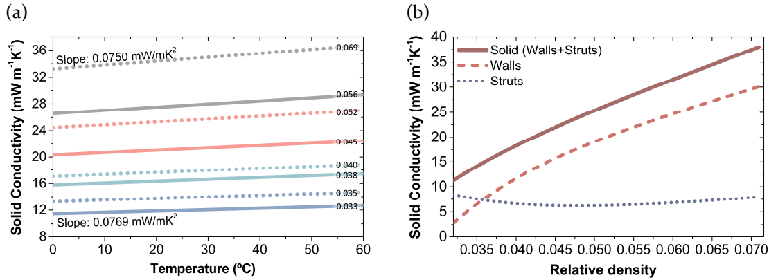
Figure 8-2-6. (a) Solid phase thermal conductivity of the foams in Table 8-2-2 as a function of temperature. (b) Thermal conductivity of the solid phase at 10 °C as a function of the relative density
