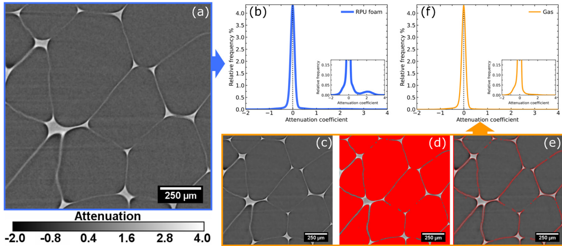
Figure 6-S1: Workflow for obtaining the solid phase attenuation density function (Figure 6-2 (b)). From the lab-scale tomography volumes (a), the attenuation density function for the foam (gas + polymer) is then calculated performing a spline interpolation to the attenuation values histogram (bin size: 0.01) (b). Next, an anisotropic diffusion filter was applied to the lab-scale tomography volumes (c), and the filtered volume was binarised to obtain the gas phase inside the cells (d). ROIs were created from the binarised volume (e) and after applying them on the original lab-scale reconstructed volumes (a) the attenuation density function of the gas could be computed (f).
