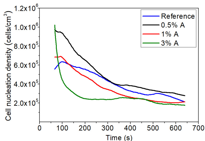
Figure 7-1-10: Cell nucleation density evolution with time for all the foams manufactured.
