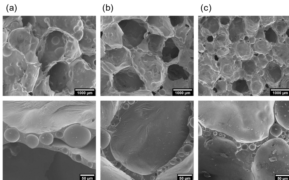
Figure 8-2-1: SEM micrographs of samples with density 92.4\ \text{kg m}^{-3} (a), 113.5\ \text{kg m}^{-3} (b) and 158.6\ \text{kg m}^{-3} (c) foams at low (first row) and high (second row) magnifications.
