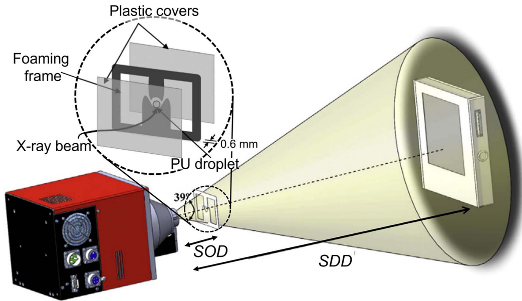
Figure 2-24: Schematic view of the X-ray radiography system used by Pardo-Alonso et al. [36]. It includes the foaming frame placed between the source and the detector.
