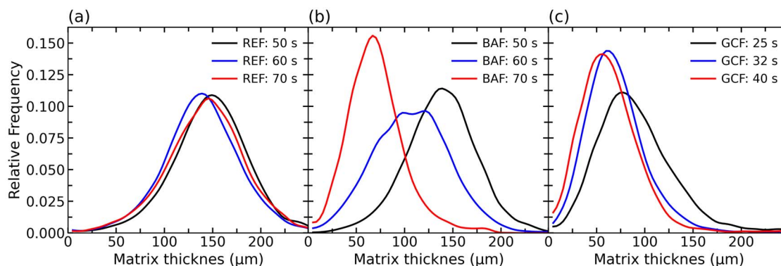
Figure 5- 5: Thickness of the solid matrix at three different reaction times for systems: (a) REF, (b) BAF, and (c) GCF.
