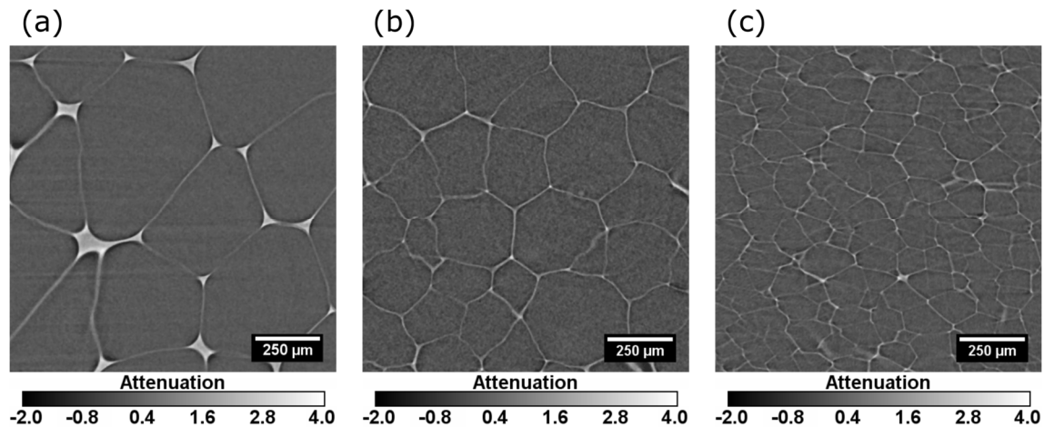
Figure 6-3: Representative laboratory X-ray tomography slices of (a) RPU, (b) LDPE, and (c) XPS foams.
