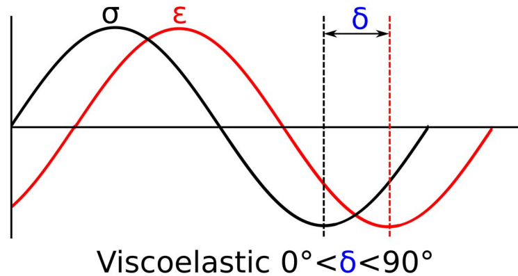
Figure 2-18: Sinusoidal behaviour of the stress, \sigma , and strain, \epsilon , for a viscoelastic material. The phase angle between both curves varies between 0^\circ and 90^\circ .
