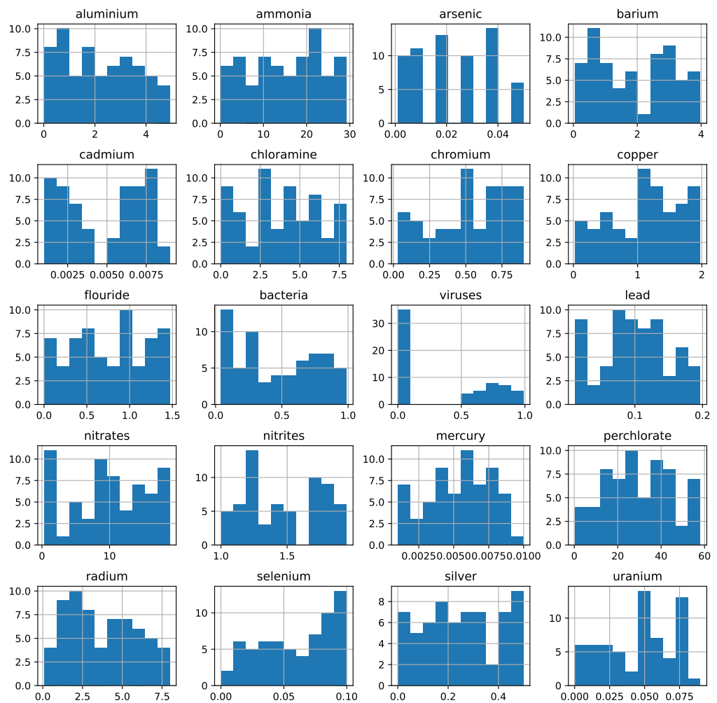
Figure 2. Distribution of water-containing compounds from the dataset.
