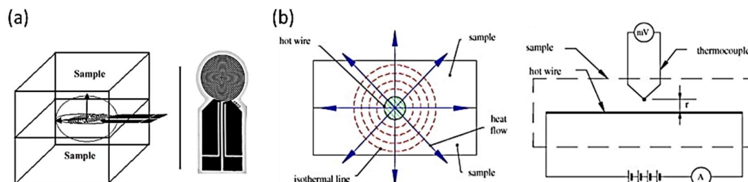
Figure 1. (a) TPS measurement scheme. Reprinted with permission from Ref. [17] Copyright © 2008 WILEY-VCH Verlag GmbH & Co. KGaA; (b) Hot wire method scheme. Reprinted with permission from Ref. [18] Copyright © 2007, Elsevier.
