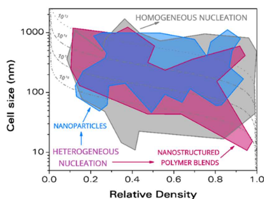
Figure 4. Comparison between the materials that have been produced taking advantage of homogeneous and heterogeneous nucleation (from reference [50]).
