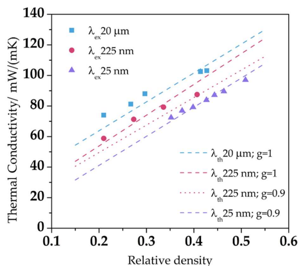
Figure 5. Experimental (points) and theoretical (dashed lines) thermal conductivities for nanocellular PMMA with different cell sizes as a function of the relative density (Adapted from reference [52]).
