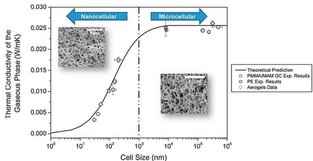
Figure 7. Gaseous thermal conductivity as a function of the cell size for different systems (Reprinted with permission from Ref. [11], Copyright © 2015, Elsevier).
