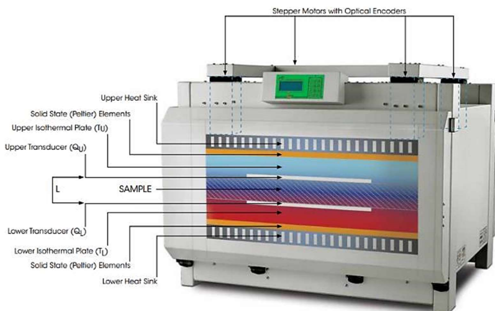
Figure 2. Heat flow meter measurement scheme [26].
