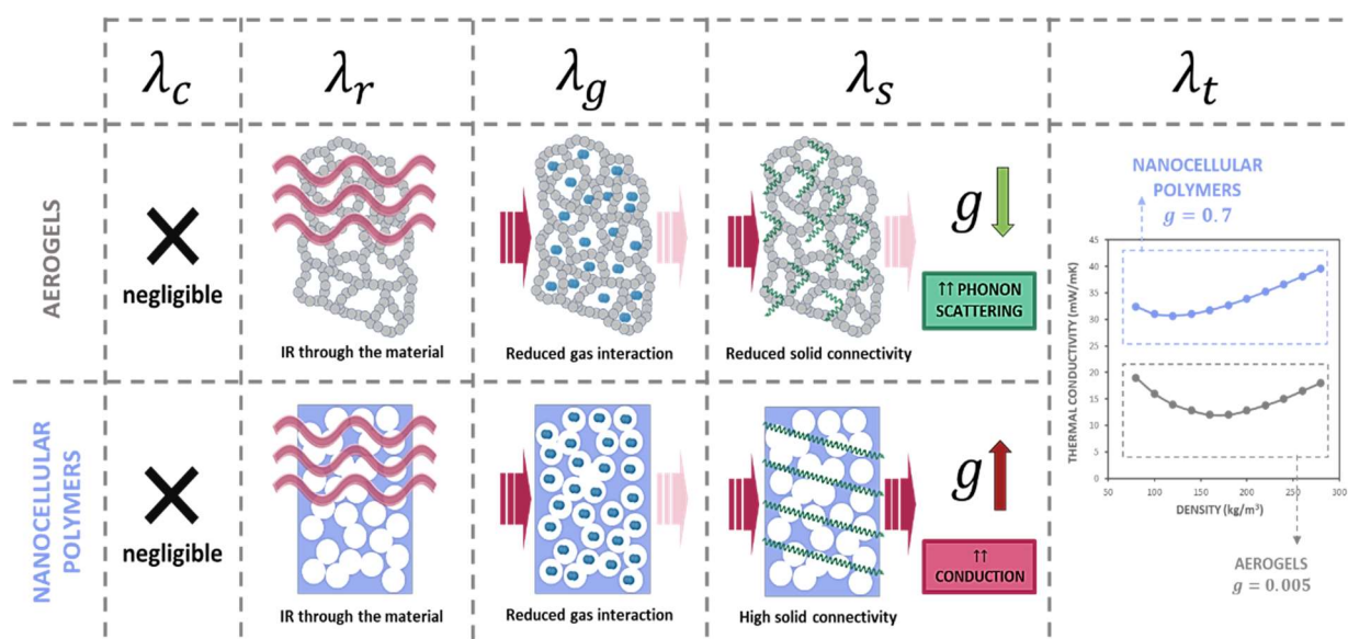
Figure 8. Heat transfer mechanisms in aerogels and nanocellular polymers. While both systems behave similarly in terms of radiation and conduction through the gas phase, there is a huge difference in the conduction through the solid material due to the intrinsic configuration of the solid phase. Nanocellular polymers show a connected solid phase, and as a result, higher conductivity.
