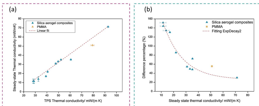
Figure 3. (a) Correlation between steady-state and TPS thermal conductivity experimental values; (b) difference percentage between TPS and steady-state methods as a function of the thermal conductivity.
