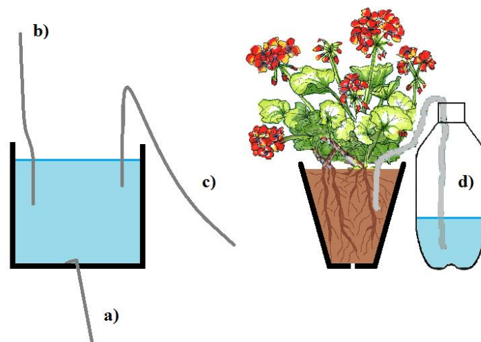
Figure 9. Slope line ( I ) of wicks: (a) downward (e.g., in the Waterboxx ® ); (b) upward (e.g., in the Wickinator ® ); (c) and (d) a combination of the two (capillary siphon); (d) typical domestic wick irrigation used for watering flower pots.
