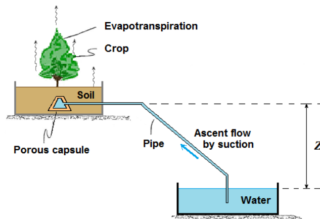
Figure 5. Pitcher irrigation system designed by Olguín [58].
