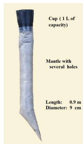
Figure 4. The “Irrigasc” permeable shaft.
