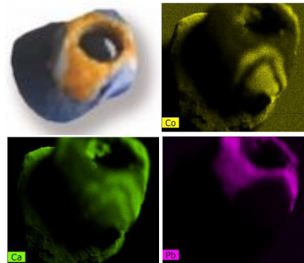
Fig. 6. Picture and X-ray fluorescence elemental compositional maps of a polychrome bead, showing the distribution of Co in the blue phase, Ca in the white phase, and Pb in the orange phase.
