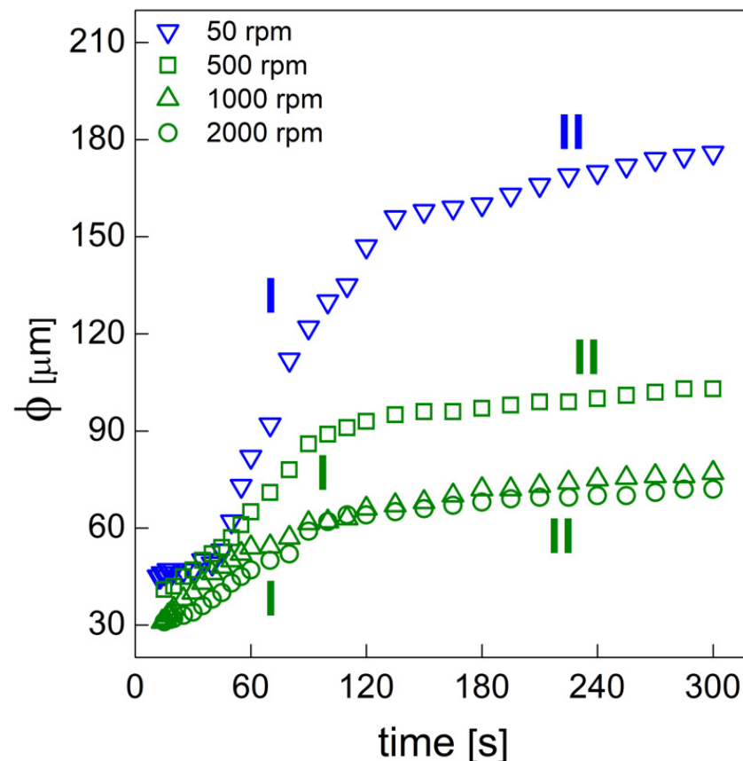
Figure 6. Bubble size evolution of the PU foams obtained at different mixing speeds.
