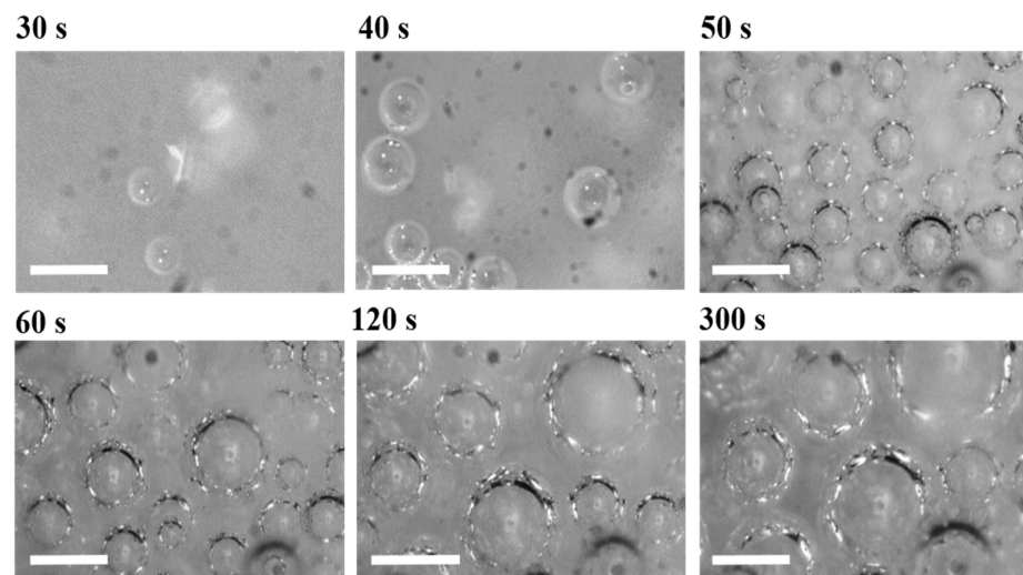
Figure 3. Microphotograms reporting the foaming process of the PU sample obtained at 50 rpm. Scale bars are 200 \mu\text{m} .
