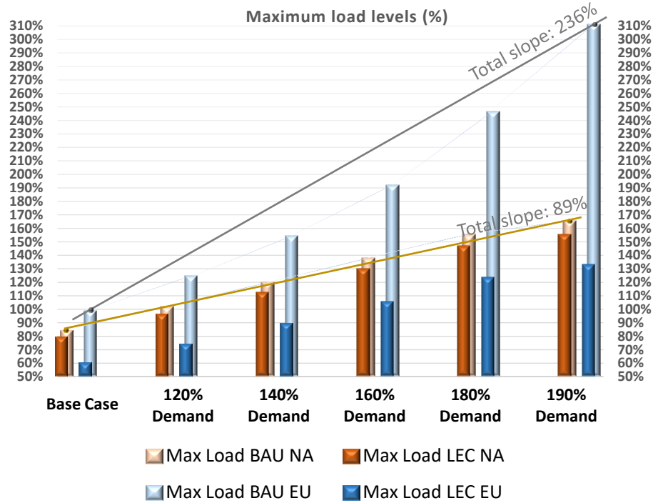
Fig. 4. Maximum load levels comparison.
