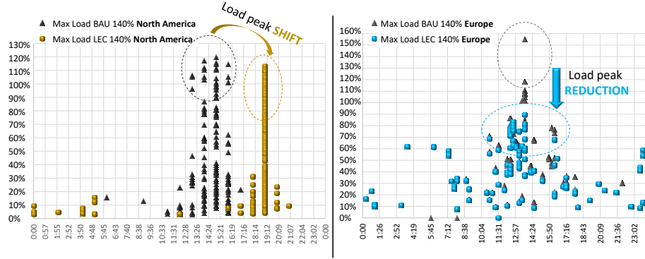
Fig. 5. Load peak hours comparison.
