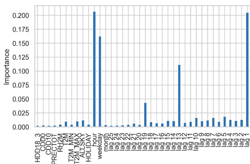
Figure 5. Random forest feature importance.
