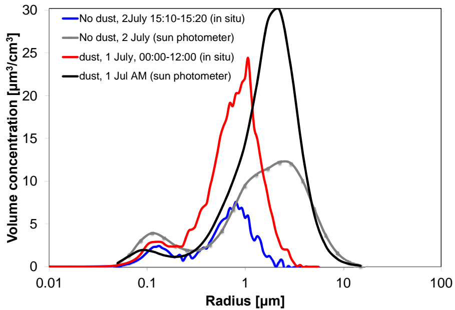
Figure 8. Volume particle size distributions for 1st July 2013 (dust case) and 2nd July 2013 (no-dust case) measured in-situ and by inversion of sun photometer data. The latter have been converted to concentration using a scale height derived from the co-located lidar observations (see details in the text).
