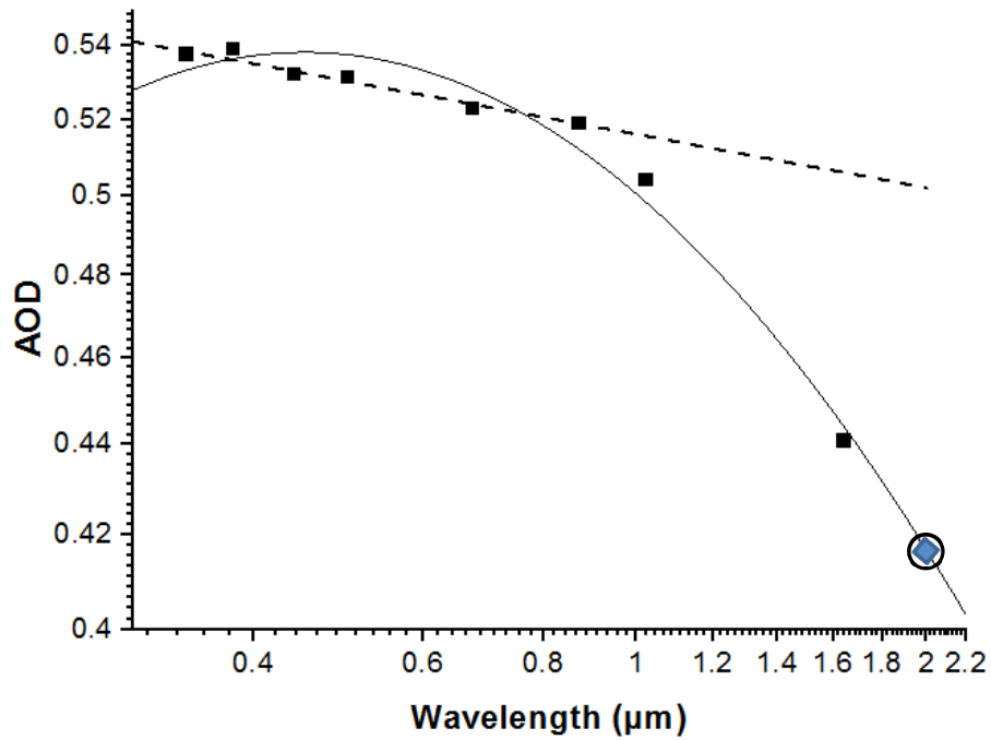
Figure 2. Aerosol optical depth as a function of wavelength in log-log scale for 11 June 2013 at 11:12UTC. Solid line indicates the 2nd order fit over the range 340-1640nm whereas the dashed line indicates the 1st order fit over the range 440-870nm, corresponding to the Ångström formula (Ångström, 1961). The extrapolated value of AOD at 2μm wavelength using the 2nd order fit is indicated with a circle.
