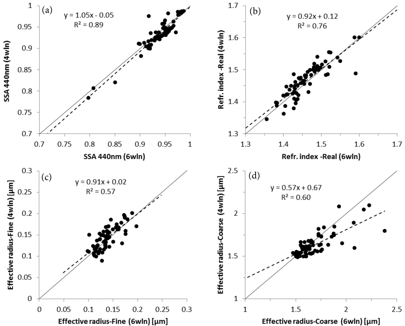
Figure 6. Comparison of inversion retrievals using 4 spectral channels (440, 675, 870, 1020nm) or 6 channels (440, 500, 675, 870, 1020 and 1640nm) in the diffuse sky radiance: (a) Single scattering albedo (440nm); (b) Real part of the refractive index; (c) Effective radius of the fine mode; (d) Effective radius of the coarse mode. Data from Cimel #789 at 'Barbados_Saltrace' using almucantar and principal plane observations.
