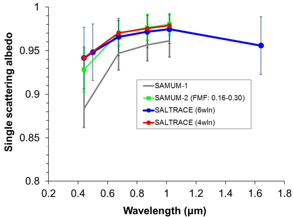
Figure 4. Single scattering albedo as a function of wavelength for SALTRACE as well as SAMUM campaigns. Average values for dust cases in each campaign are provided. Bars indicate \pm 1 standard deviation. For SAMUM-2 only cases with low fine mode fractions (FMF) between 0.16 and 0.30 are considered. For SALTRACE data, retrievals using 6 wavelength (6wln) and 4 wavelength (4wln) channels are shown.
