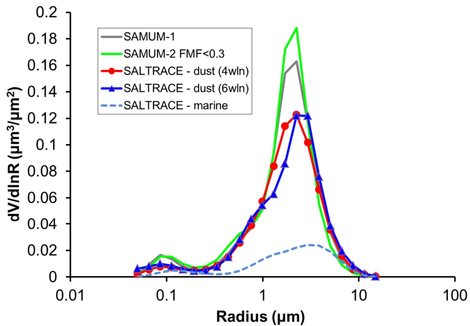
Figure 5. Volume particle size distributions ( dV/d\ln R ) for SALTRACE as well as SAMUM campaigns. Average values for dust cases in each campaign are provided. For SAMUM-2 only cases with low fine mode fractions (FMF) between 0.16 and 0.30 are considered.
