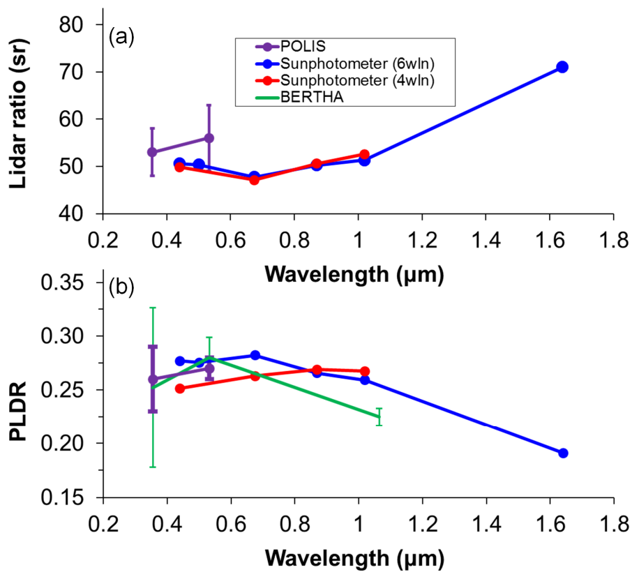
Figure 7. Wavelength dependence of (a) lidar ratio (LR); (b) Particle linear depolarization ratio (PLDR), for dust cases during SALTRACE. Data from POLIS lidar (Groß et al., 2015) and BERTHA lidar (Haarig et al., 2017) are compared to the 4-wavelength and 6-wavelength sun photometer retrievals. Vertical bars in lidar data indicate uncertainty due to systematic errors.
