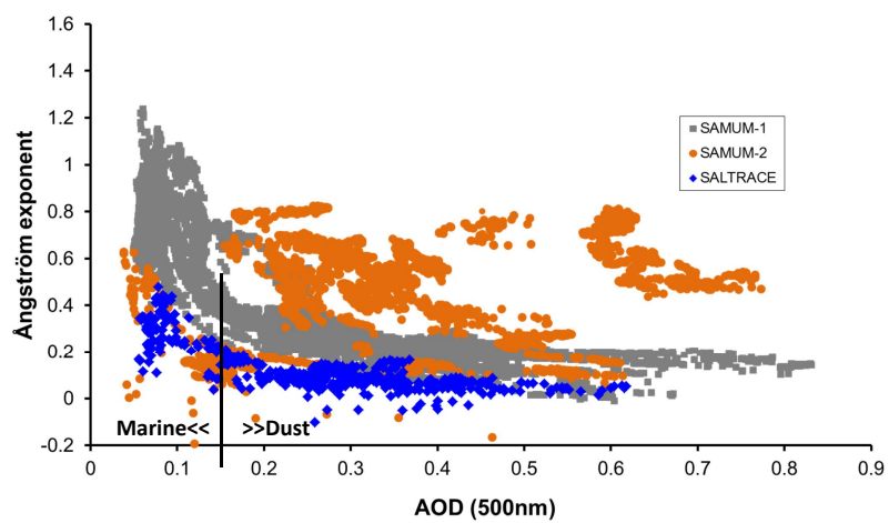
Figure 3. Scatter plot of Ångström exponent vs. aerosol optical depth (500nm) for SALTRACE as well as SAMUM-1 and SAMUM-2 campaigns.
