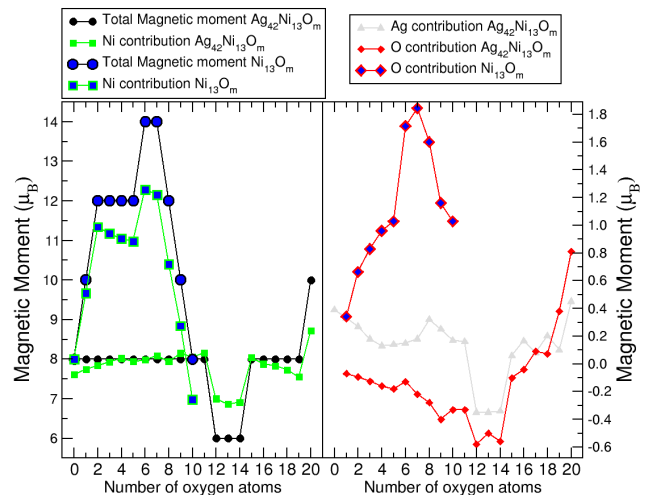
FIG. 5. (Color online) Contribution of the different atomic species to the total magnetic moment of the magnetic nanoparticles.
