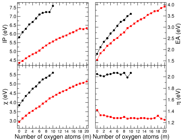
FIG. 6. (Color online) Indicators of global reactivity. Panel (a) vertical ionization potential (IP), panel (b) electronic affinity (EA), panel (c) electronegativity ( \chi ) and panel (d) chemical hardness ( \eta ). The black line corresponds to \text{Ni}_{13}\text{O}_m , while the red line represents \text{Ni}_{13}@Ag_{42}\text{O}_m .
