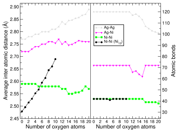
FIG. 3. (Color online) Average inter-atomic distances (left panel) and number of atomic bonds (right panel) for \text{Ni}_{13}@\text{Ag}_{42}\text{O}_m as functions of the oxygen content. In black, the Ni-Ni values for \text{Ni}_{13}\text{O}_m . We consider that two neighboring atoms form a bond when their inter-atomic distance is smaller than the average distance of those atoms in the non-oxidized system plus 10%.
