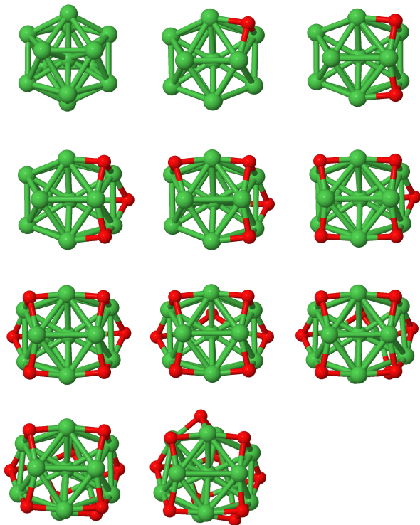
FIG. 2. (Color online) Putative ground state atomic configurations of \text{Ni}_{13}\text{O}_m with m= 1 to 10 .
