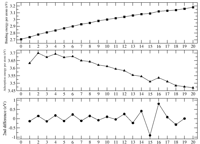
FIG. 4. (Color online) Binding energy per atom (upper panel), oxygen adsorption energy (central panel), and second energy difference (lower panel) of \text{Ni}_{13}@\text{Ag}_{42}\text{O}_m as a function of the oxidation rate.
