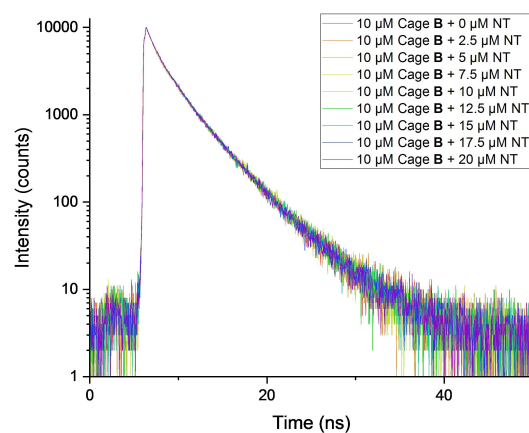
Figure 6. Fluorescence lifetime profile (excited at 375 nm) of cage B (10 \mu\text{M} ) in 2:8 of THF/H 2 O and different NT concentrations.
