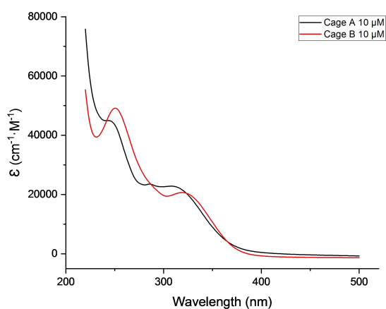
Figure 3. UV spectra of cages A and B (10 \mu\text{M} ) in 2:8 THF/ \text{H}_2\text{O} .
