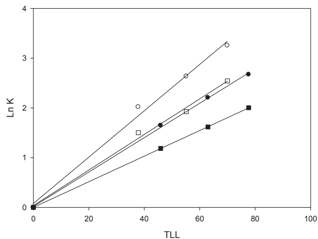
Fig. 4. Logarithm of the partition coefficients of the flavonoids versus tie-line length for: (○) quercetin on {EL (1) + sodium citrate (2) + water (3)}, (□) quercetin on {EL (1) + potassium citrate (2) + water (3)}, (●) rutin on {EL (1) + sodium citrate (2) + water (3)}, (■) rutin on {EL (1) + potassium citrate (2) + water (3)} and (-) fits from equation (10) at T = 298.15\text{ K} and at p = 101.3\text{ kPa} .
