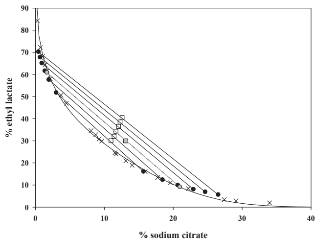
Fig. 3. Comparison of tie-line compositions obtained in this work (black) and tie-line compositions reported by Kamalanathan et al. [20] (grey) for the ternary system {ethyl lactate (1) + sodium citrate (2) + water (3)}. Symbols: (□) feed compositions, (X) binodal curve, (●) tie-line data and (-) fit of the binodal data by eq.1 at T = 298.15\text{ K} and p = 0.1\text{ MPa} .
