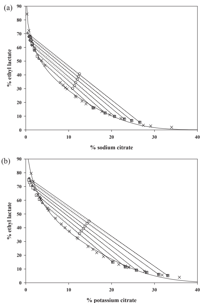
Fig. 2. Binodal curves and corresponding tie-lines for the ternary systems containing ethyl lactate, salt and water at T = 298.15 K and p = 0.1 MPa. (○) feed compositions, (X) binodal curve, (---) fit of the binodal data, (●, grey) experimental tie-line compositions and (□) calculated tie-lines compositions using the UNIQUAC model. (a) {EL (1) + sodium citrate (2) + water (3)}; (b) {EL (1) + potassium citrate (2) + water (3)}.
