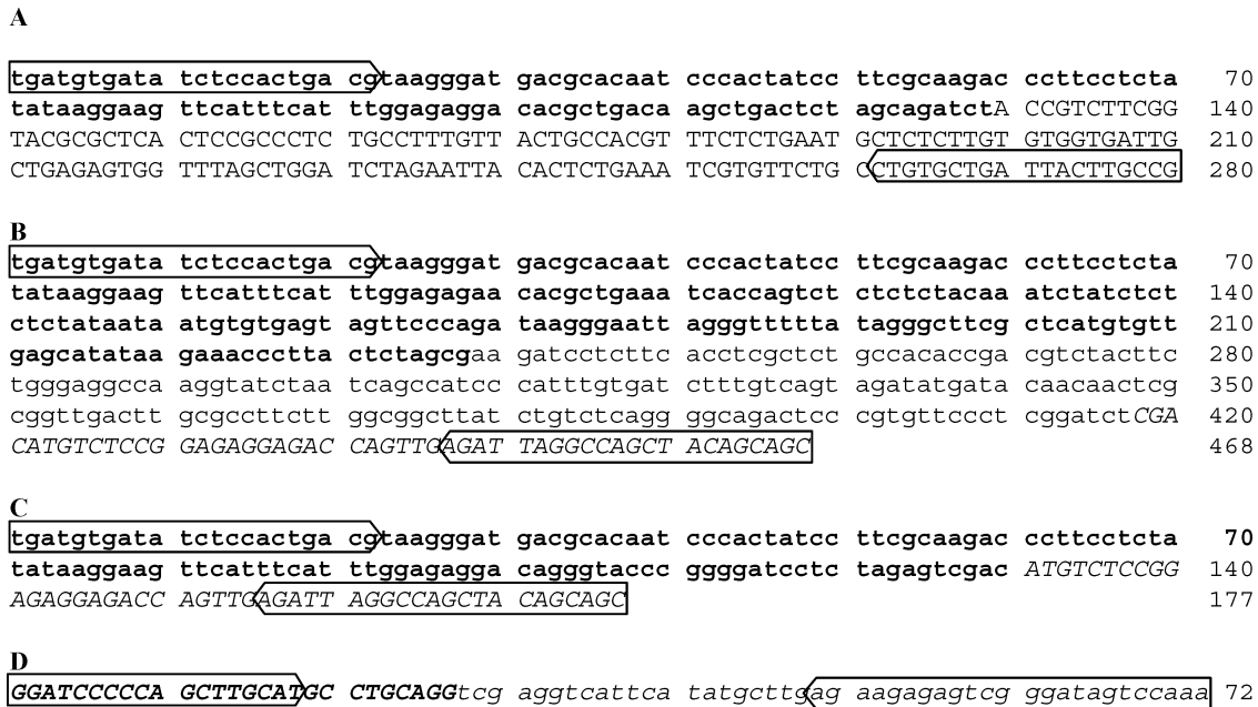
Figure 1. DNA sequences from the MON810 (A), Bt11 (B), T25 (C), and GA21 (D) events amplified with the described PCR method. Primers are boxed, with arrows indicating the orientation. Lowercase letters highlighted in bold indicate the sequence of the 35S promoter; capital letters, the hsp70 intron; lowercase letters, the Adh1 gene; capital letters and italics, the PAT gene; capital letters in bold and italics, the plasmid flanking sequence; and lowercase letters in italics, the 5' sequence of the act-r promoter.
