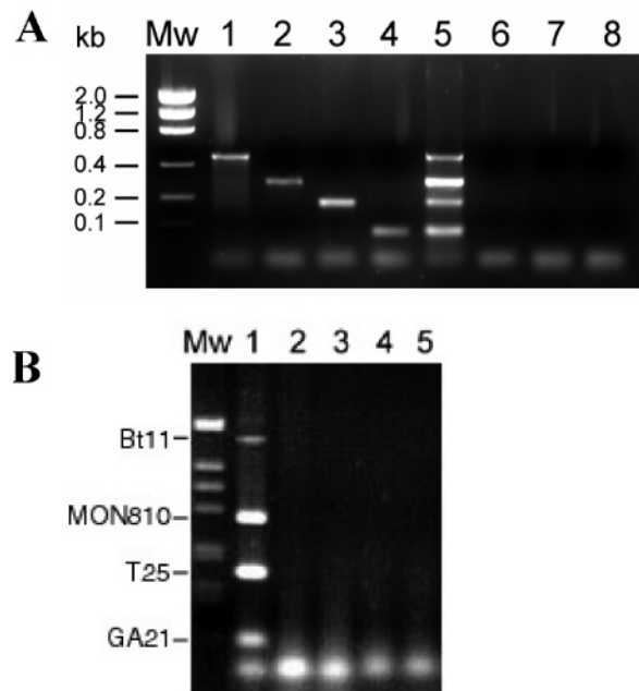
Figure 3. GMO amplification with the multiplex PCR method. (A) Amplification with the target maize GMs: lane 1, Bt11 (468 bp); lane 2, MON810 (280 bp); lane 3, T25 (177 bp); lane 4, GA21 (72 bp); lane 5, mixture of the four transgenic DNAs; lane 6, wild-type maize; lane 7, wild-type soybean; lane 8, no template control. (B) Control of amplification with nontarget GMOs: lane 1, amplification of the four target GMO; lane 2, Bt176 maize; lane 3, RR soybean; lane 4, RR cotton; lane 5, StarLink maize. 1% dilutions of each of these DNAs were used as template.
