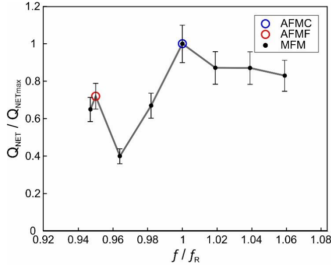
FIG. 7. The net flow rate non-dimensionalized with its maximum value as a function of the pinching frequency for values close to the resonant frequency. The blue circle shows the automatic frequency mode by capacitance. The red circle indicates the automatic frequency mode by flowmeter. Each data point is calculated by averaging the net flow rate and the resonant frequency of 121 consecutive cycles. Error bars represent one standard deviation.
