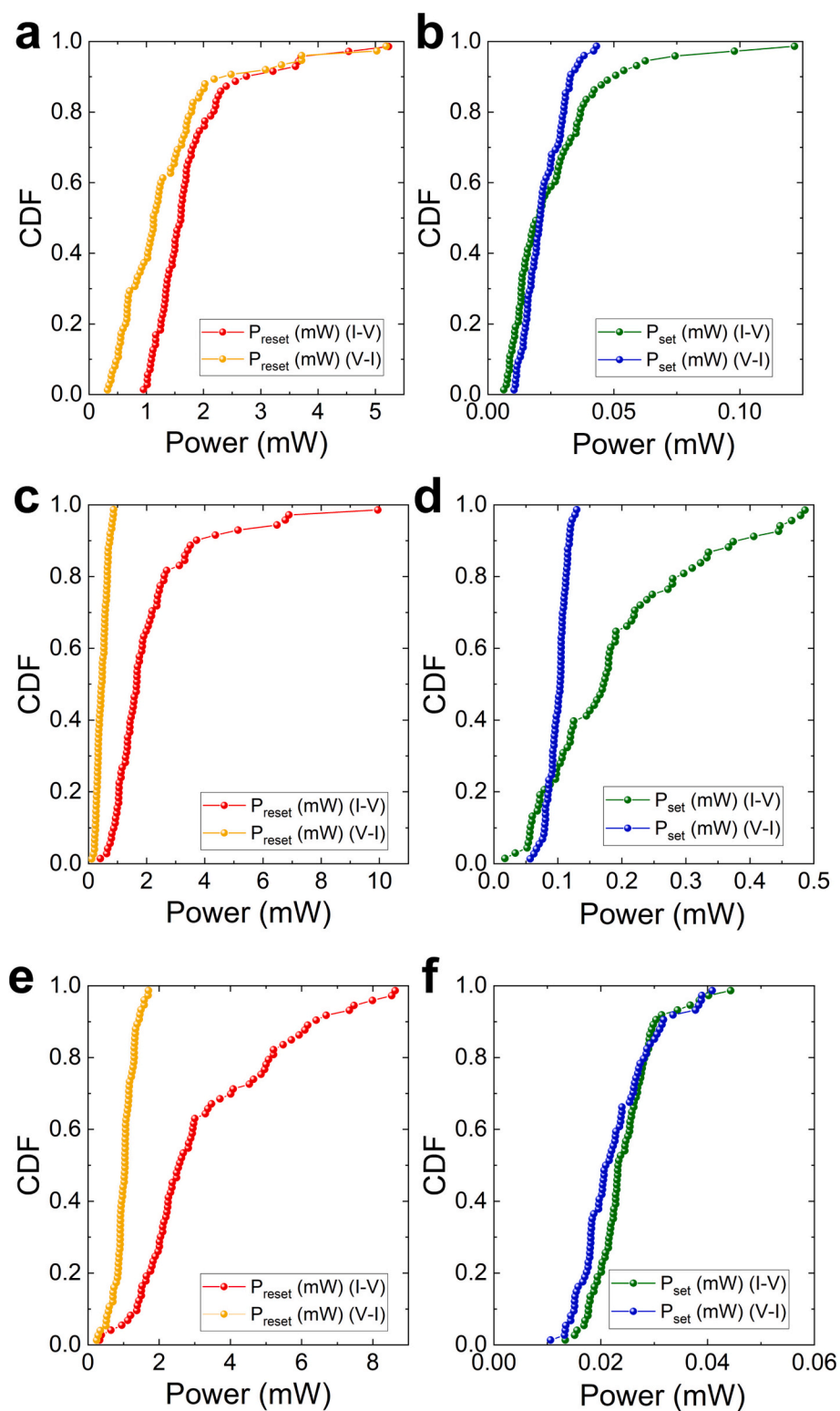
Fig. 7. Cumulative distribution functions for the power consumption for both reset (left column) and set (right column) transitions for Ni/HfO 2 /Si-n + (a - b), Ni/HfO 2 /Al 2 O 3 /Si-n + (c - d) and Ni/HfO 2 /Al 2 O 3 /HfO 2 /Al 2 O 3 /HfO 2 /Si-n + (e - f) samples. Panels (a, c, e) show the power absorbed by the reset transition when applying voltage (red) and current (yellow). Panels (b, d, f) show the power absorbed by the set transition when applying voltage (green) and current (blue). (For interpretation of the references to colour in this figure legend, the reader is referred to the web version of this article.)
