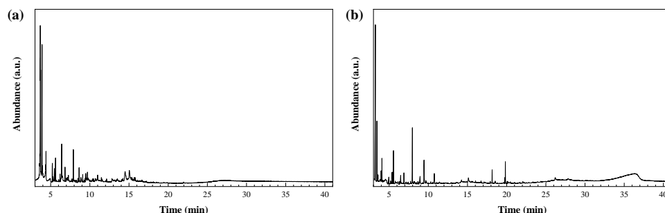
Figure 1. GC-MS chromatograms of S. aspera (a) leaf and (b) fruit hydromethanolic extracts.
