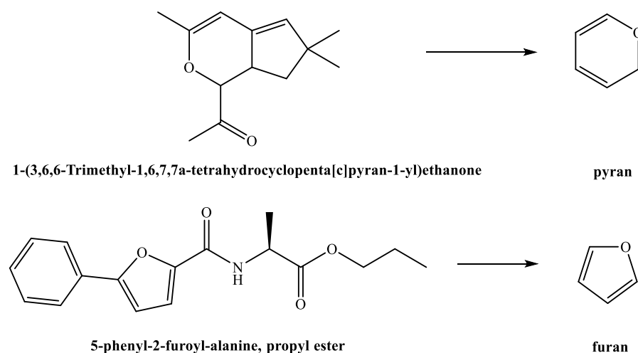
Figure 12. Suggested pyran and furan precursors.
