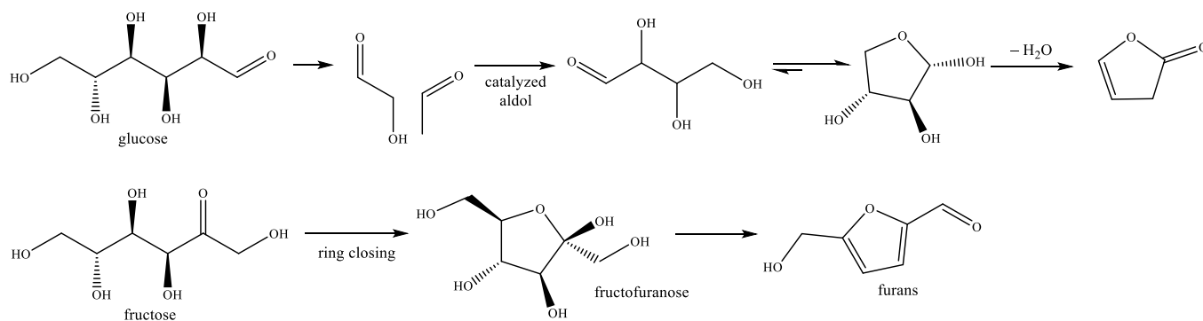
Figure 13. Proposed pathways for the transformation of carbohydrate-derived products into furans.
