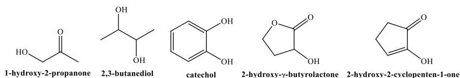
Figure 4. Chemical structures of some of the chemical species identified in both S. aspera leaf and fruit extracts.
