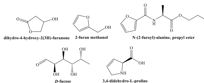
Figure 3. Structures of some of the chemical species found in S. aspera fruit extract.
