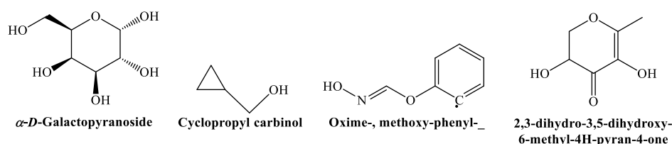
Figure 2. Structures of some of the chemical species found in S. aspera leaf extract.
