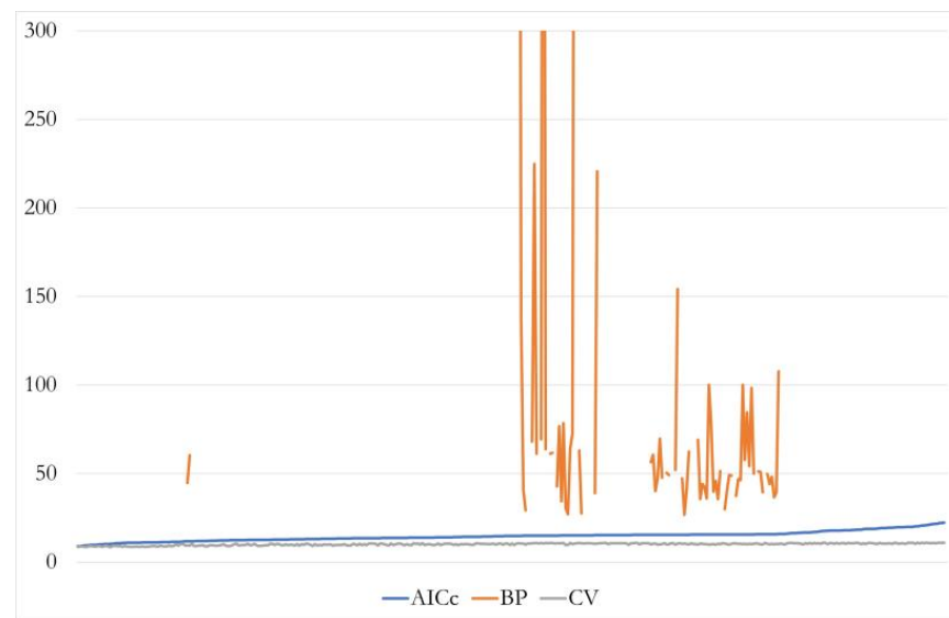
Figure 4. Condition numbers obtained according to different conceptualizations of distance.
