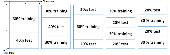
Fig. 7. Representation of the five block-division train-test partitions employed in the study.
