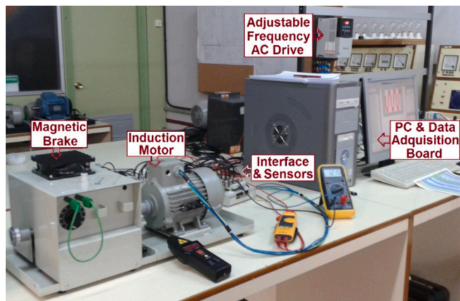
Fig. 9. Test bench.
