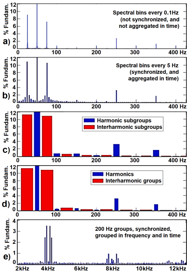
Fig. 11. Different representations of the frequency spectrum of the PowerFlex inverter output current with scalar control and PWM modulation, exciting an induction motor with eccentricity.
