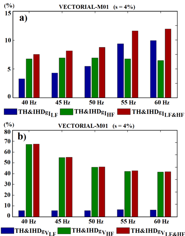
Fig. 14. Relationships between harmonic and interharmonic rates of low frequency TH&IHD gILF , high frequency TH&IHD gIHF and total high and low frequency TH&IHD gILF&HF , when changing the fundamental output frequency, for current (a), and voltage (b).
