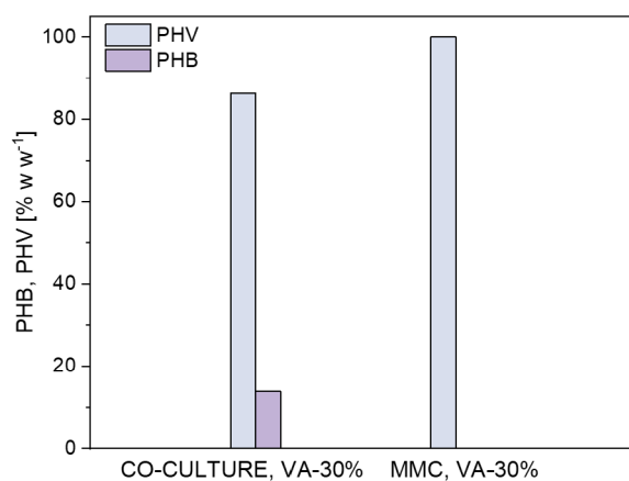
Figure 3. Average PHAs composition obtained with valeric acid supplemented at 30% w w -1 of the total carbon during the cultivation of synthetic cocultures and the mixed methanotrophic consortium.
