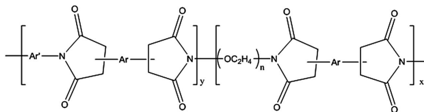
Aromatic-aliphatic copoly(ether-imide)
