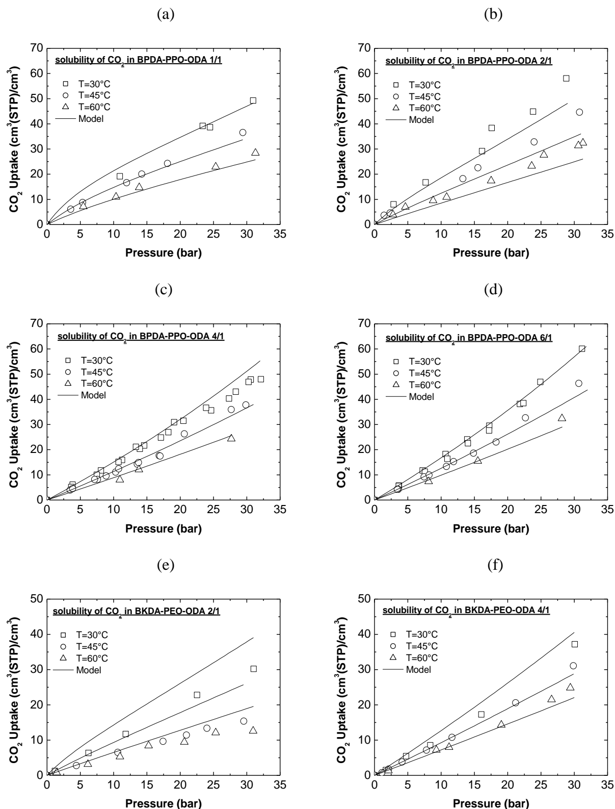
Fig. 14: Comparison between experimental solubility data and modelled solubility data with LF and NELF models in BPDA-PPO-ODA 1/1 (a), 2/1 (b), 4/1 (c), 6/1 (d) and BKDA-PEO-ODA 2/1 (e) and 4/1 (f) at 30^\circ\text{C} , 45^\circ\text{C} and 60^\circ\text{C} .
