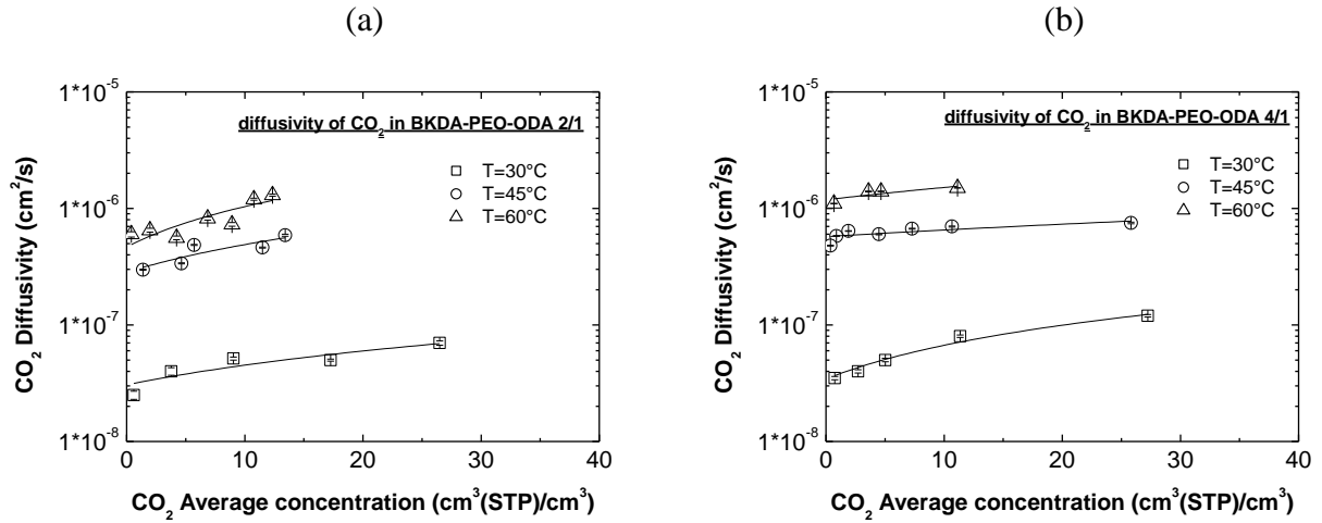
Fig.8: The effect of temperature on CO 2 diffusivity in BKDA-PEO6000-ODA 2/1 (a), 4/1 (b). Solid lines are data interpolations.
