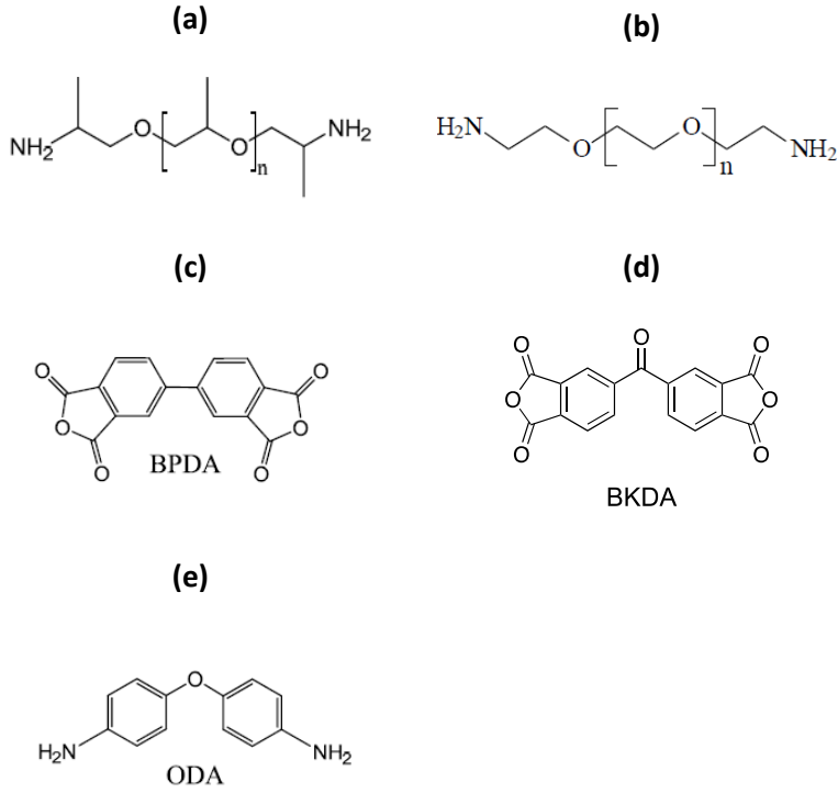
Fig.1: Structure of (a) diamino-terminated PPO, (b) diamino-terminated PEO, (c) BPDA, (d) BKDA and (e) ODA [6,7]
