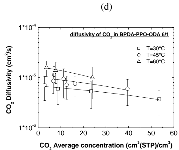
Fig. 4: The effect of temperature on \text{CO}_2 diffusivity in BPDA-PPO4000-ODA 1/1 (a), 2/1 (b), 4/1 (c) and 6/1 (d) samples. Solid lines are data interpolations.
