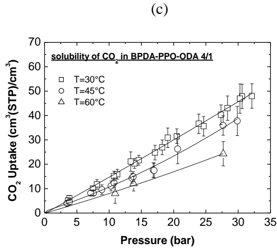
Fig. 3: The effect of temperature on \text{CO}_2 solubility isotherms in BPDA-PPO4000-ODA 1/1 (a), 2/1 (b), 4/1 (c) and 6/1 (d) samples. Solid lines are data interpolations.
