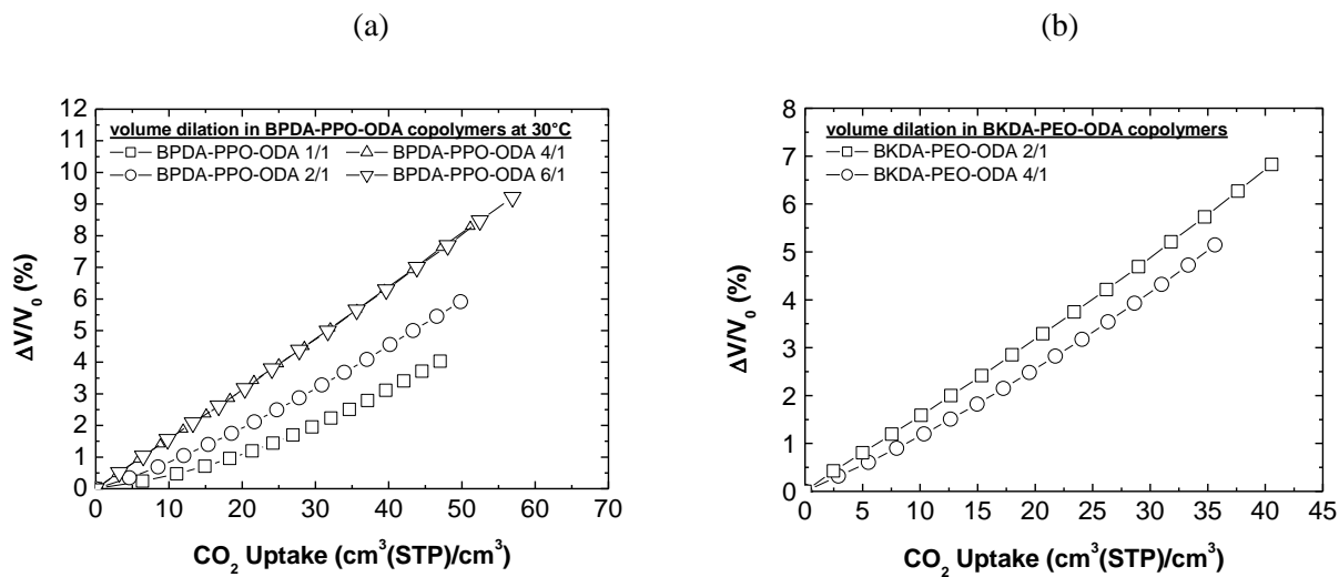
Fig. 15: Calculation of volume dilation in BPDA-PPO-ODA (a) and BKDA-PEO-ODA (b) at 30^\circ\text{C} with LF model
