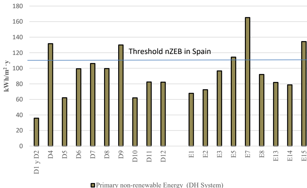
Fig. 11. EI_{p,nr} , biomass DHS ( \text{kWh}/\text{m}^2 \cdot \text{y} ).
