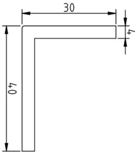
Figure 44: Dimensions L-profile
