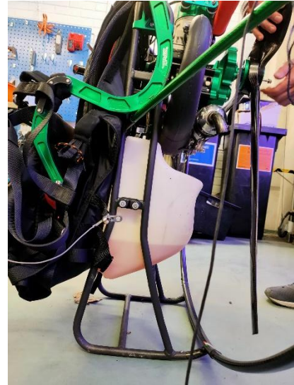
Figure 52: Side view of the paramotor
