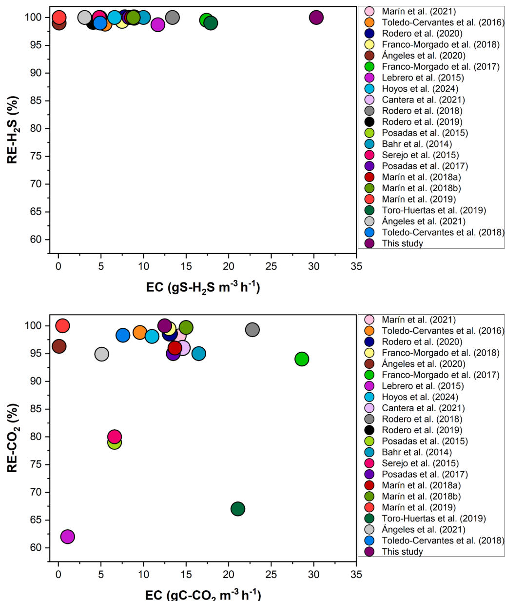
Fig. 3. Summary of the performance of previous studies assessing the simultaneous removal of (a) H 2 S and (b) CO 2 in pilot and lab-scale algal photobioreactors. Legend: RE – removal efficiency, LR – loading rate. Parameters were directly taken from the referenced studies when reported. When not explicitly provided, they were calculated based on the available data within the respective papers.
